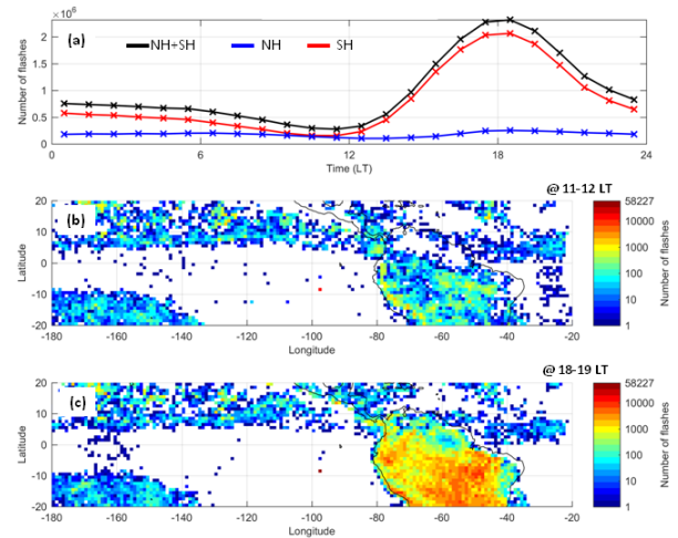
Figure 9. 2-year (2020-2021) December lightning distribution recorded by the two GLM sensors with (a) total number of flashes recorded between 20S and 20N latitudes, (b) distribution of flashes between 11 and 12 Local Time (LT), and (c) same as (b) but for 18-19 LT.
