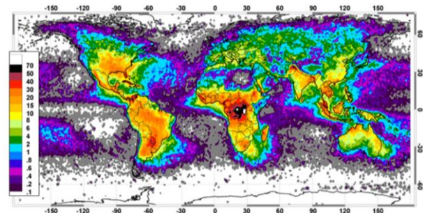
Figure 1. Annual average number of lightning flashes per km 2 from NASA low orbit LIS and OTD missions, adapted from [2].
