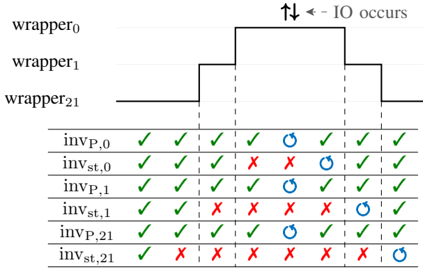
Figure 17: Overview of when different invariants need to hold when invoking wrapper 21 in our first example, where \circlearrowleft denotes an invariant being reestablished for a new view of the trace.
