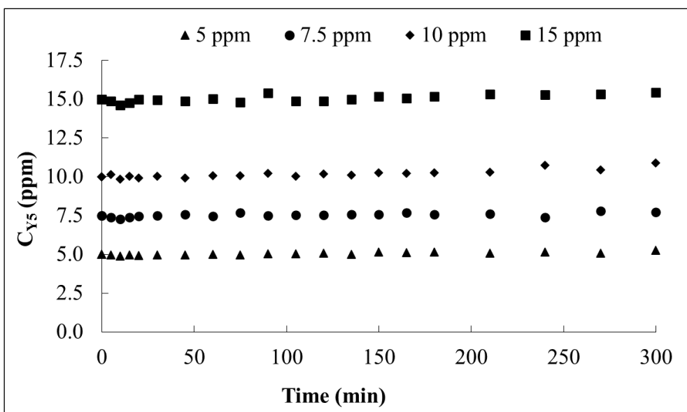
Figure S6. Direct photolysis of dye Y5 under artificial solar light (i.e., using a solar simulator) as a function of the initial concentration of the dye; a catalyst loading of 1 \text{ g L}^{-1} was used.
