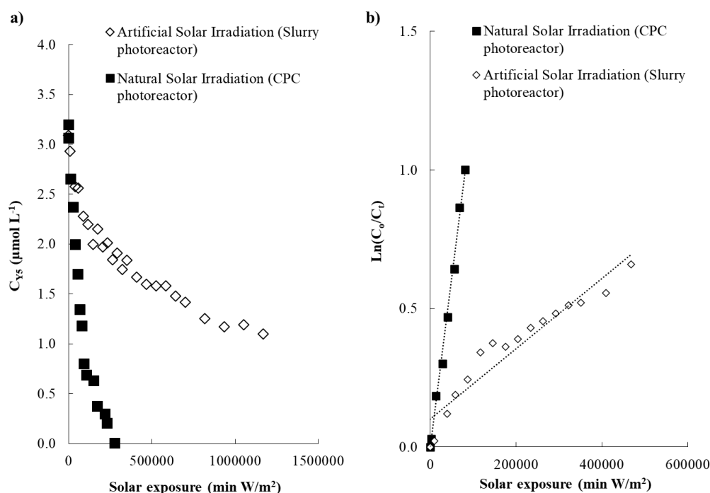
Figure 7. a) Kinetic disappearance of Y5 on Cu@C catalyst as a function of the solar exposure ( \text{min} \cdot \text{W} \cdot \text{m}^{-2} ) under natural solar irradiation and artificial solar light (symbols); b) first-order linear fitting of the kinetic data (lines).
