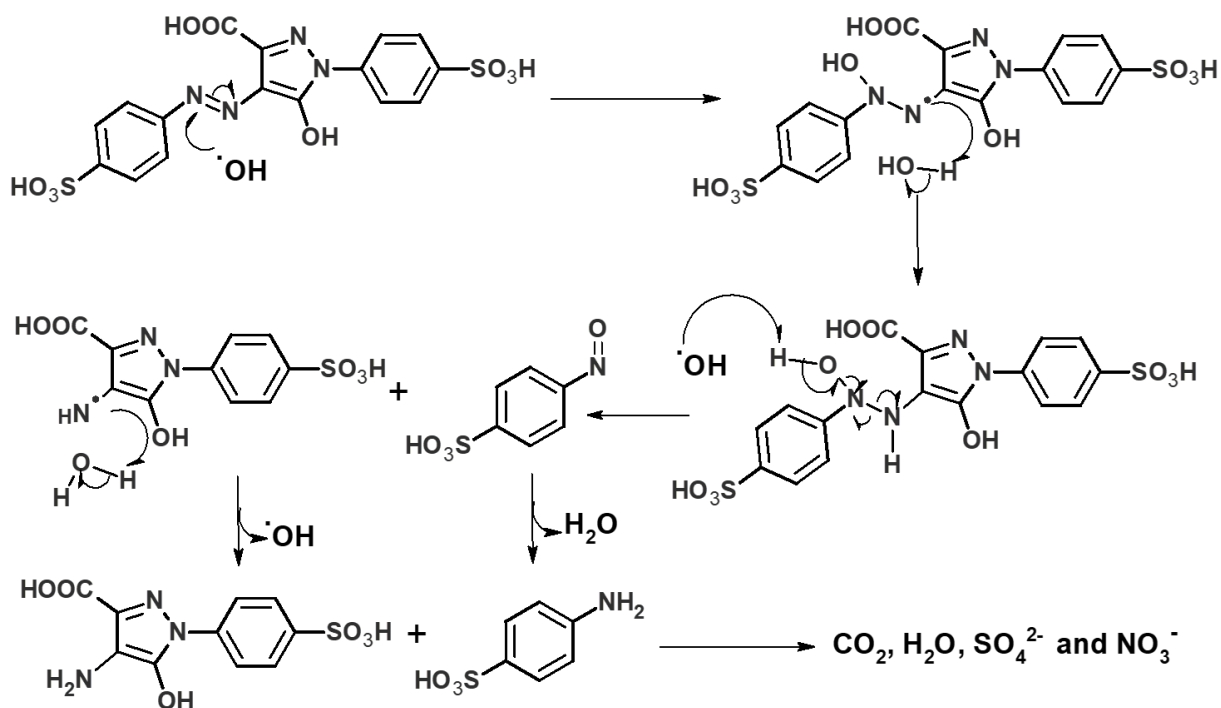
Figure 10. Proposed mechanism for the Y5 degradation under natural solar irradiation.
