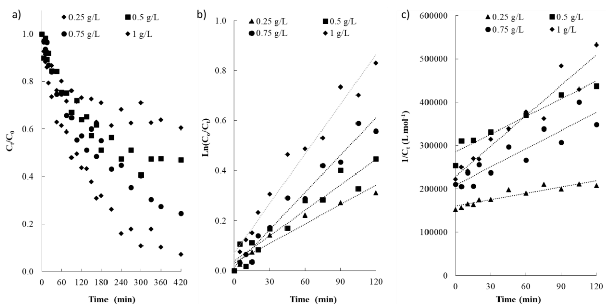
Figure 4. a) Kinetics of Y5 photodegradation under artificial solar light at various Cu@C catalyst loadings for an initial concentration of 5 ppm of the dye (symbols); b) first-order, and c) second-order reaction-rate linear representation (lines) of the experimental data.
