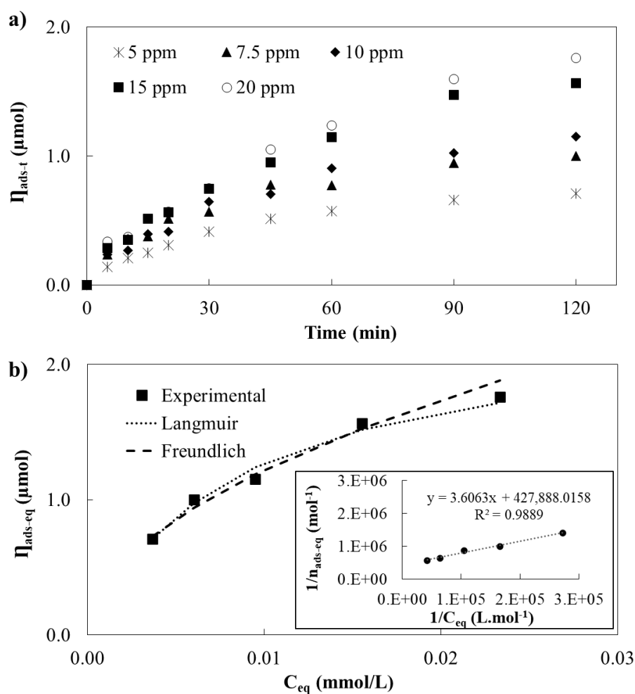
Figure 3. a) Kinetics of Y5 adsorption in the dark for a Cu@C catalyst loading of 1 \text{ g}\cdot\text{L}^{-1} ; b) Experimental equilibrium adsorption isotherm (symbols) and fitting to Langmuir and Freundlich models (lines). Inset: Linear regression according to Langmuir's model.
