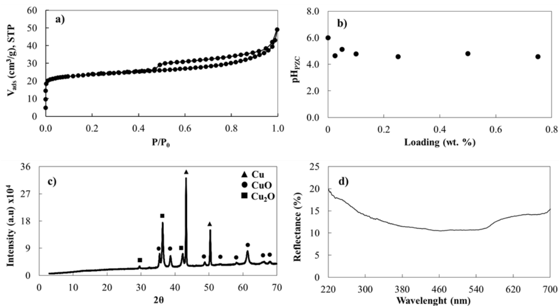
Figure S4. Physicochemical characterization of Cu@C catalyst. a) N 2 adsorption-desorption isotherms at -196 °C; b) Surface pH; c) XRD pattern; d) UV-Vis/DR spectra.
