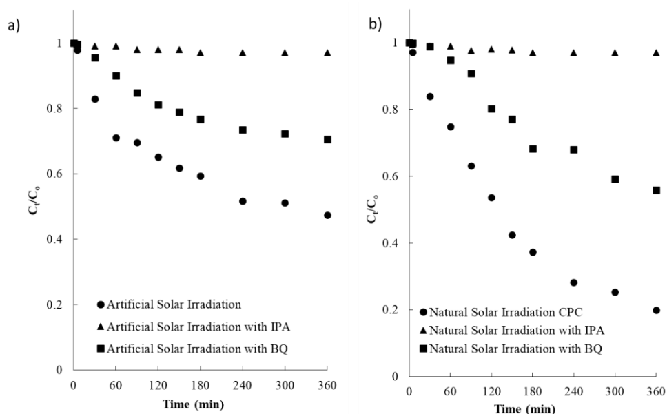
Figure 9. Kinetics of Y5 photodegradation on Cu@C photocatalyst in the absence and presence of IPA and BQ scavengers: a) Artificial solar light; b) natural solar light.
