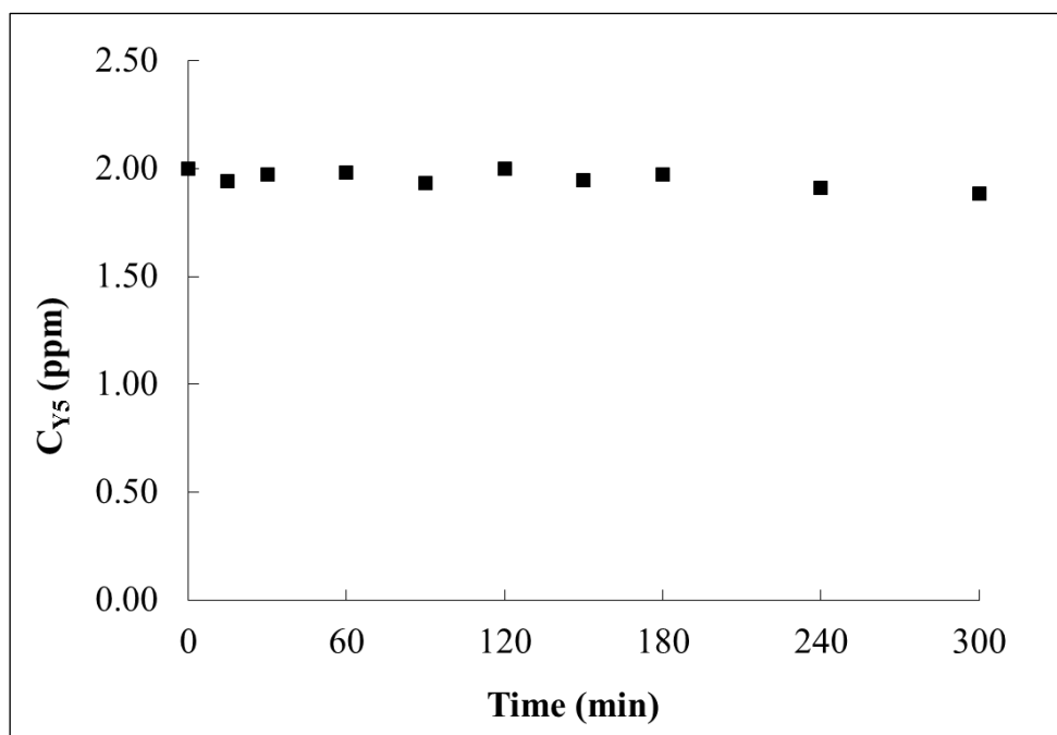
Figure S8. Direct photolysis of dye Y5 under simulated UV-VIS light. Initial concentration of the dye was 2 ppm.
