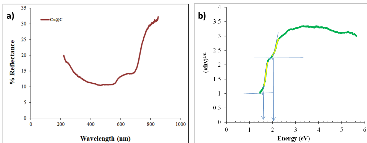
Figure S5. a) UV-Vis diffuse reflectance spectrum of the Cu@C photocatalyst. b) Tauc graphical representation with indication of the two optical features used for the estimation of the band gap.
