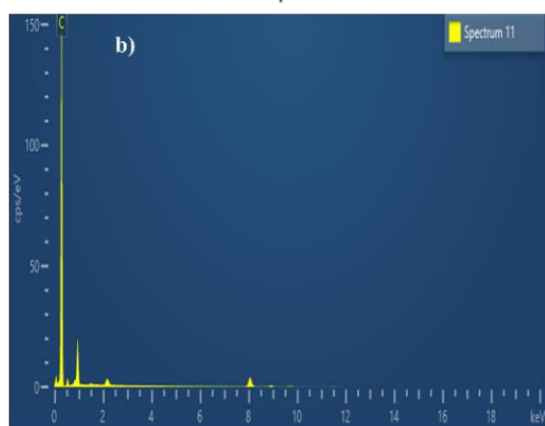
Figure S2. a): SEM image; b): EDS analysis; and c): ED pattern of Cu@C catalyst.
