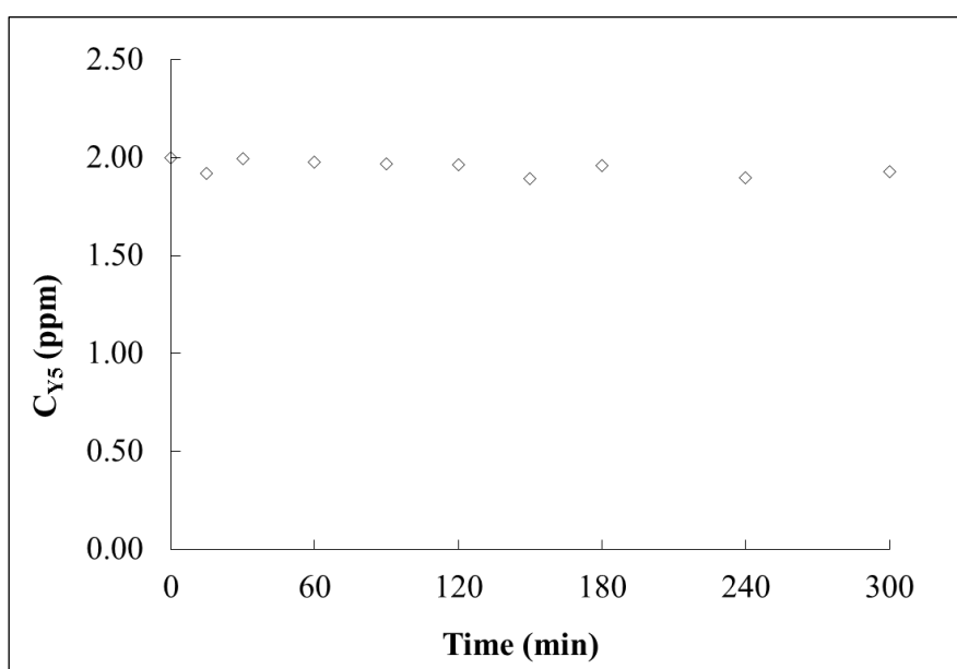
Figure S7. Direct photolysis of dye Y5 under sunlight using a CPC reactor. Initial concentration of the dye was 2 ppm.
