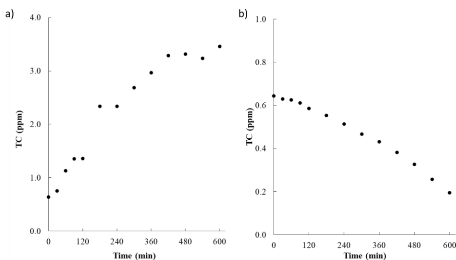
Figure 8. Total carbon (TC) evolution detected during the photodegradation of yellow 5 on irradiated Cu@C photocatalyst: a) artificial solar light; b) natural solar light. Experimental conditions: 2 ppm Y5 and 0.25 g L -1 catalyst loading.
