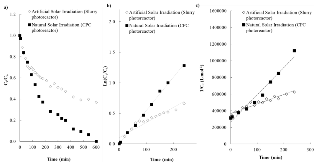
Figure 6. Comparison of the photocatalytic activity of Cu@C catalyst under artificial and natural solar light using two photoreactor configurations: a CPC photoreactor and a slurry photoreactor. Catalyst loading was fixed to 0.25 \text{ g L}^{-1} and initial concentration of the dye to 2 ppm; a) Kinetics of Y5 concentration in the photocatalytic assays (symbols); b) First-order, and c) Second-order linear fitting (lines) of the kinetic data.
