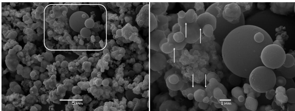
Figure 1. SEM images of Cu@C catalyst.
