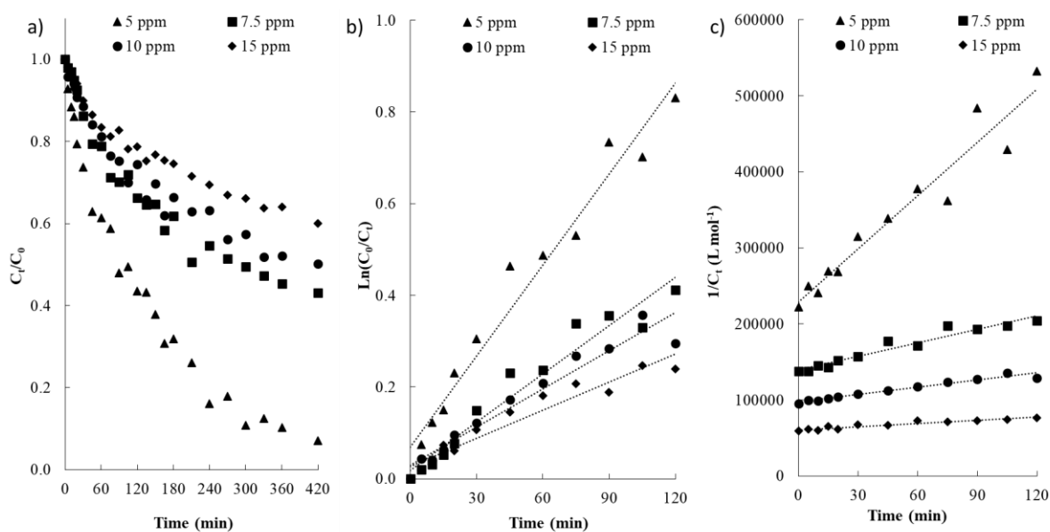
Figure 5. a) Kinetics of Y5 photodegradation under artificial solar degradation for a catalyst loading of 1 \text{ g L}^{-1} and varied initial concentrations (symbols); b) first-order, and c) second-order linear fitting (lines) of the kinetic data.
