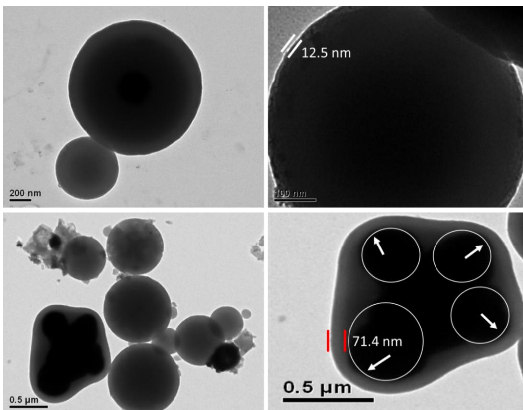
Figure 2. Selected TEM images of Cu@C catalyst.
