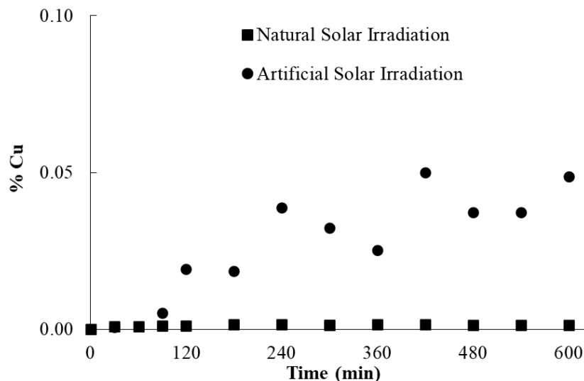
Figure 11. Copper lixiviation under artificial and natural solar irradiation.
