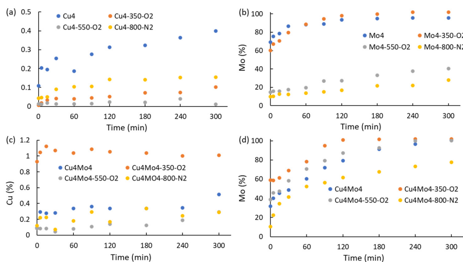
Figure 10. Kinetics of Cu and Mo lixiviation from catalysts under artificial solar irradiation. (a) Cu series; (b) Mo series; (c) Cu in CuMo series; (d) Mo in CuMo series.
