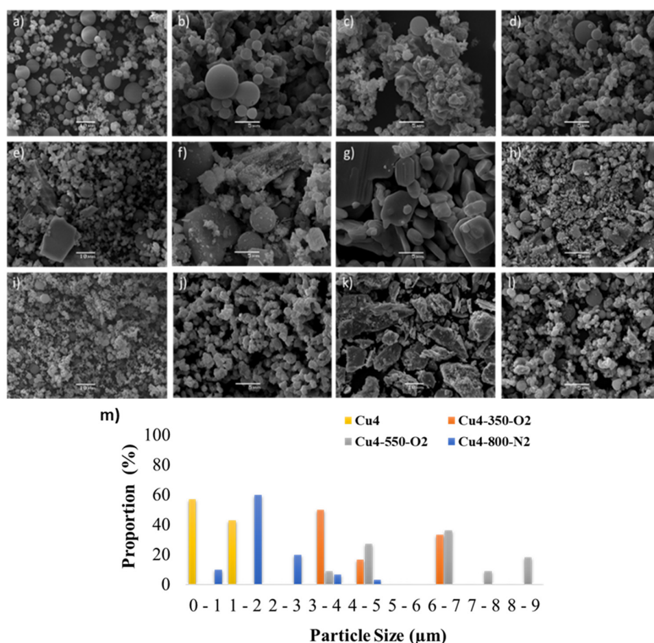
Figure 1. Scanning electron microscopy images. (a) Cu4; (b) Cu4-350-O 2 ; (c) Cu4-550-O 2 ; (d) Cu4-800-N 2 ; (e) Mo4; (f) Mo4-350-O 2 ; (g) Mo4-550-O 2 ; (h) Mo4-800-N 2 ; (i) Cu4Mo4; (j) Cu4Mo4-350-O 2 ; (k) Cu4Mo4-550-O 2 ; (l) Cu4Mo4-800-N 2 . (m) Histogram for the Cu-based catalysts.
