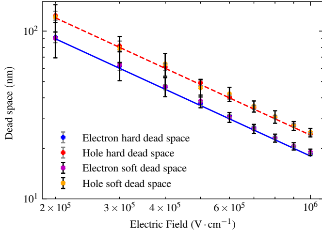
Fig. 3. Extracted dead space at various electric fields for hard and soft threshold models. Error bars represent the 99% confidence intervals. Plain blue and red lines represent theoretical values from formula (14) for electron and hole, respectively. Both models give values close to the theoretical calculation with an expected higher variability for the soft dead space model.
