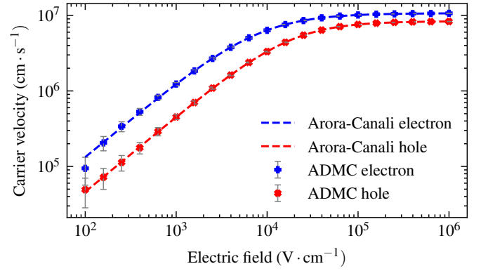
Fig. 1. Comparison of the carriers' drift velocity between input model [21], [22] and the Monte-Carlo results. Error bars represent the 99% confidence interval. The velocity is extracted by computing the distance over time ratio for 1000 electrons at different electric fields. The results show that our algorithm reproduces perfectly the input mobility model at any electric field.
