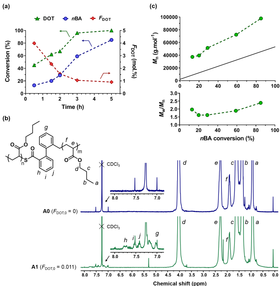
Figure 3. Synthesis of PAA- b -P( n BA-co-DOT) nanoparticles by copolymerization of n BA and DOT in water at 110 °C initiated by a PANA 20 -SG1 macroalkoxyamine ( A1 , Table 1): (a) evolution of n BA conversion, DOT conversion and average molar fraction of DOT ( F_{DOT} ) in the copolymer vs. time; (b) ^1H NMR spectrum (400 MHz, CDCl_3 ) in the 0–8 ppm region of PAA- b -P( n BA-co-DOT) copolymers A0 and A1 ; (c) evolution of M_n and \bar{D} vs. n BA conversion.
