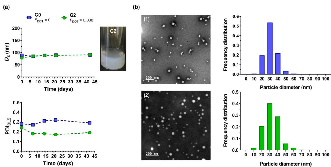
Figure 6. Colloidal properties of PAA- b -P(S-co-DOT) nanoparticles ( G0 and G2 , Table 1). (a) Variation of the intensity-average diameter ( D_z ) and polydispersity index ( PDI_{DLS} ) with time measured by DLS. (b) Representative TEM images and associated size distribution ( n = 500 ) for nanoparticles: (1) G0 and (2) G2 .
