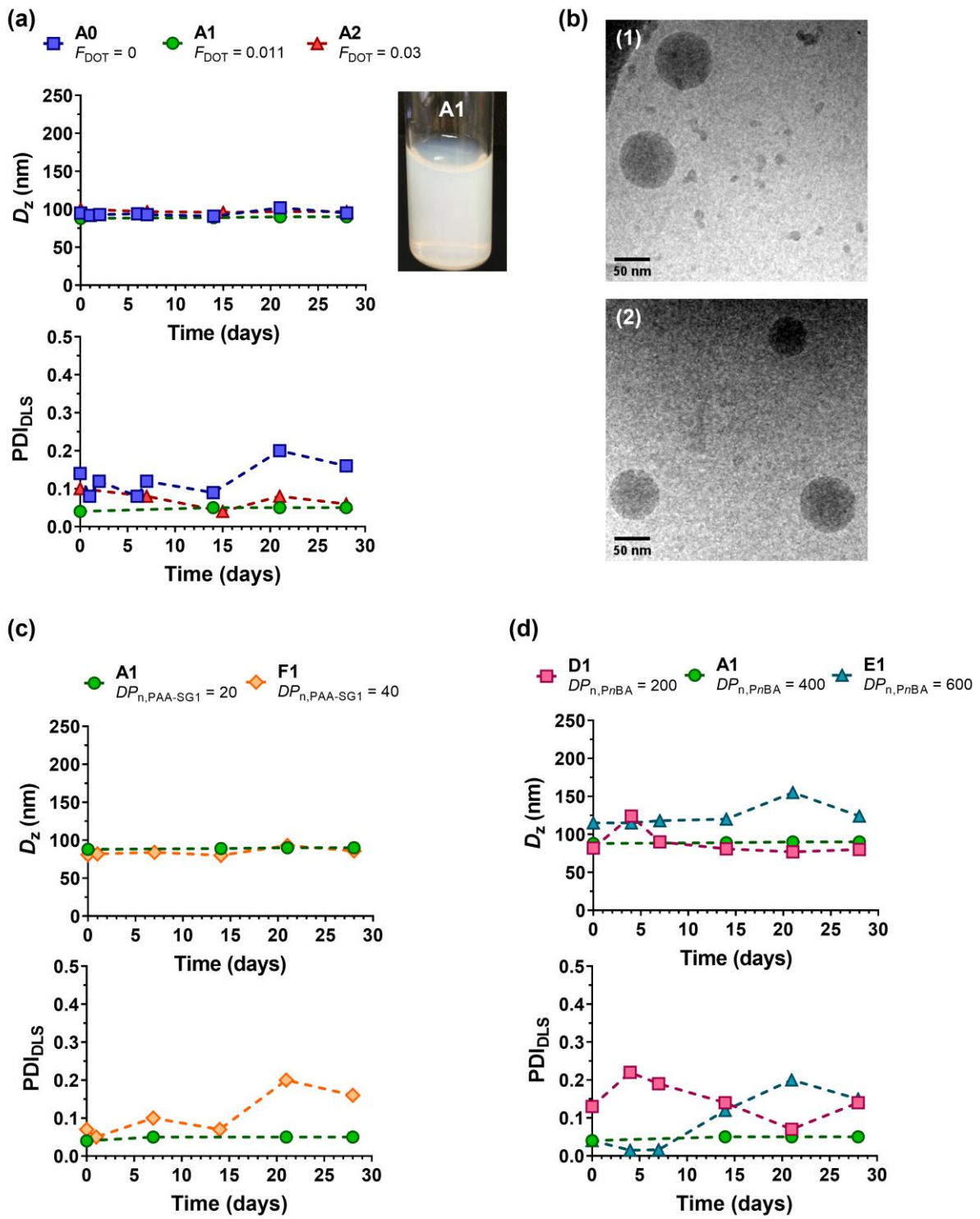
Figure 4. Colloidal properties of PAA- b -P( n BA-co-DOT) nanoparticles ( A0 , A1 , A2 , D1 , E1 and F1 , Table 1). Variation of the intensity-average diameter ( D_z ) and polydispersity index ( PDI_{\text{DLS}} ) with time measured by DLS as function of: (a) F_{\text{DOT}} , (c) DP_{n,\text{PAA-SG1}} and (d) DP_{n,\text{PrBA}} . (b) Representative cryo-TEM images of nanoparticles: (1) A0 and (2) A1 (Table 1). Note that the small objects in presence of nanoparticles are ice crystals.
