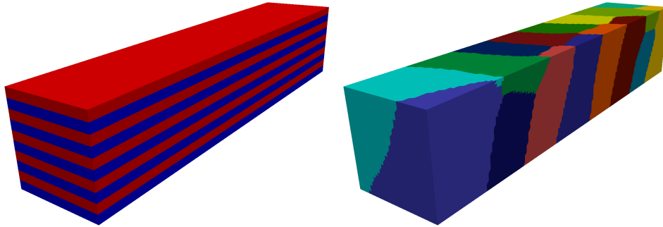
FIGURE 5.1. Heterogeneous beam composed of 10 alternating layers of rubber material (E_1, \nu_1) = (1.10^7, 0.4999) and steel material (E_2, \nu_2) = (2.10^9, 0.35) . Coefficient distribution (left) and mesh partitioning into 16 subdomains by the automatic graph partitioner Metis (right).
