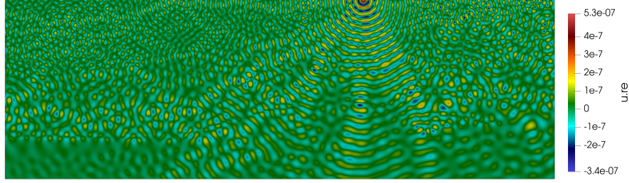
Fig. 2 The real part of the solution to the Marmousi problem at 20 Hz. The domain is 9.2 km×3 km.
