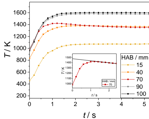
Fig. 2. T(t) recorded by the 0.20 mm S-type thermocouple at 15, 40, 70, 90 and 100 mm HAB.
