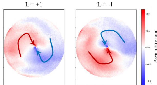
Figure 1. Example of magnetic helicoidal dichroism. For a given value L of the orbital angular momentum, the scattered intensity in the far field is collected for the two opposite winding senses of the vortex magnetization. Each panel represents, for a given L , the difference of the two intensity maps divided by their sum.
