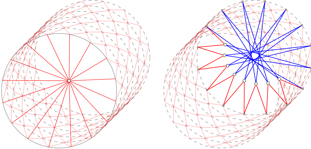
Figure 10: BM(\ell, 2k)
