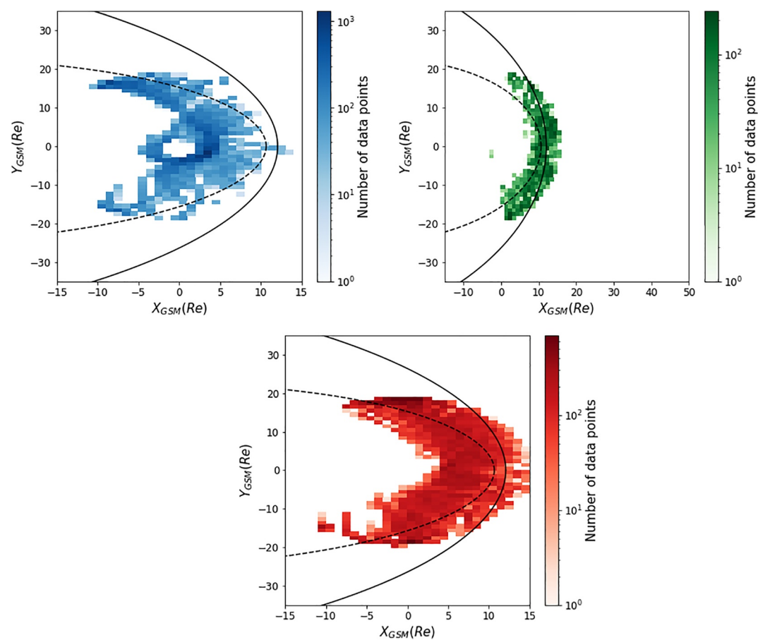
Figure A3. Spatial coverage of the Cluster labeled data set. The legend is the same than in Figure 2.
