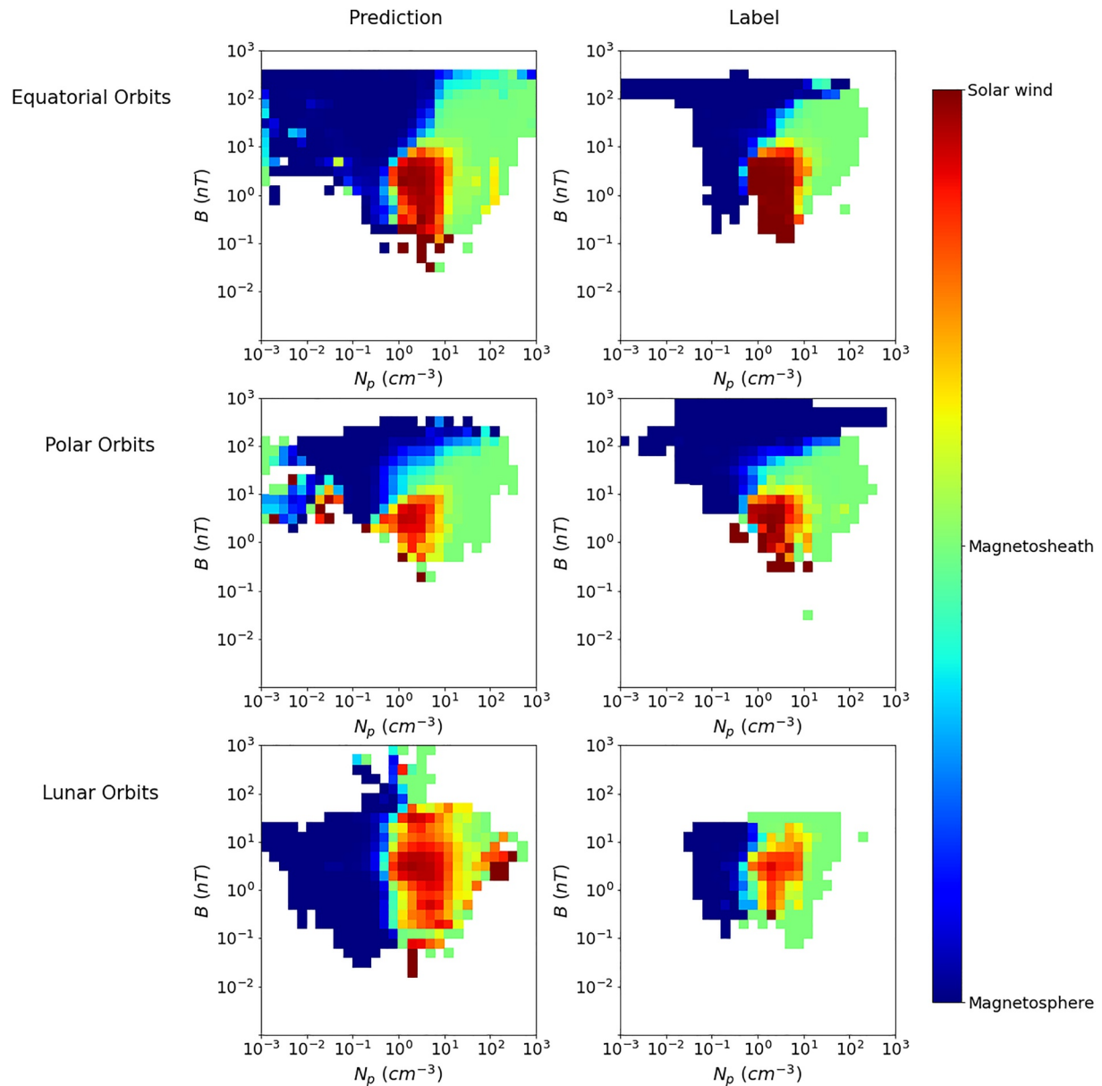
Figure 10. Binned average of the massive prediction ( left column ) and the training label ( right column ) of the equatorial ( first row ), the polar ( second row ) and the lunar ( third row ) models projected in the ( N_p , B ) plane.
