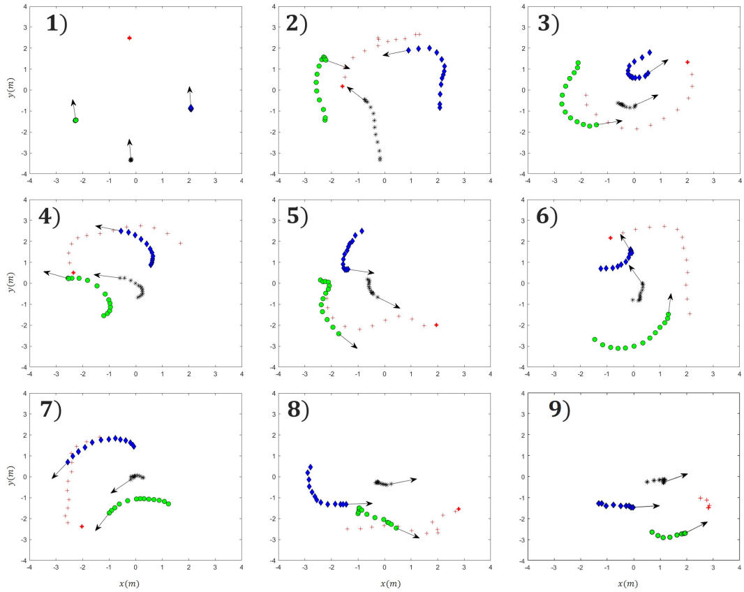
Fig. 13. Real-time performance when three aerial drones pursuit an aerial intruder drone with random movements.
