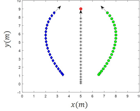
Fig. 6. Trajectories generated for three agents and a fixed target. The pursuers start in the bottom of the square and they pursuit the target with constant velocity. The deviation offset ( \alpha_0 ) for this pursuit is 30 degrees.
