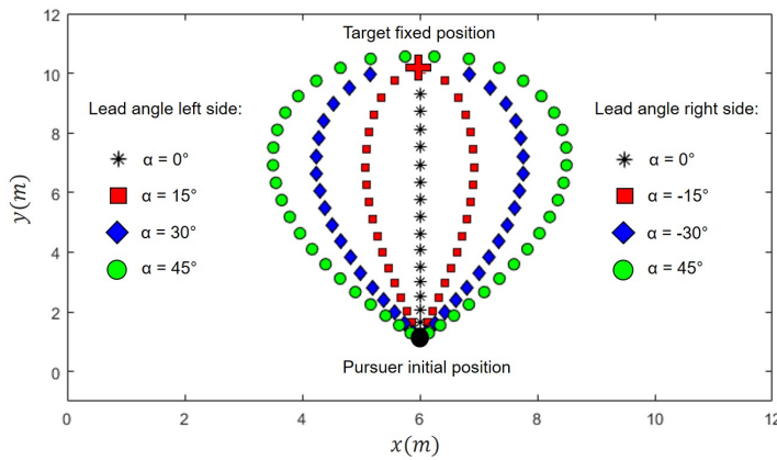
Fig. 3. Paths of deviated pursuit agents according to different angle offsets \alpha . The agents begin the trajectory at a fixed position, given by the black dot and keep a constant velocity until reaching the target.
