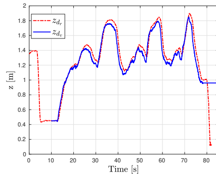
Fig. 12: x, y, z -position performances of the virtual drone and the real vehicle obtained from the first scenario. Observe the good behavior of the real drone when imitates the virtual drone trajectory.
