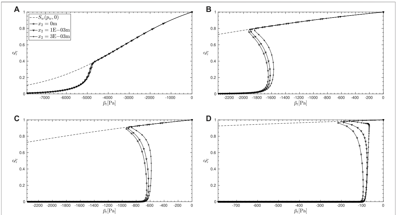
FIGURE 5 | Path followed by the solution in the space (S_t, p_t) at the boundary x_2 = 0\text{m} and two locations within the domain close to this boundary for values of w_1 (A) 2000 \text{ N}\cdot\text{m}^{-3} (B) 1000 \text{ N}\cdot\text{m}^{-3} , (C) 500 \text{ N}\cdot\text{m}^{-3} , and (D) 100 \text{ N}\cdot\text{m}^{-3} . The dashed line represents the standard non-degraded retention curve.
