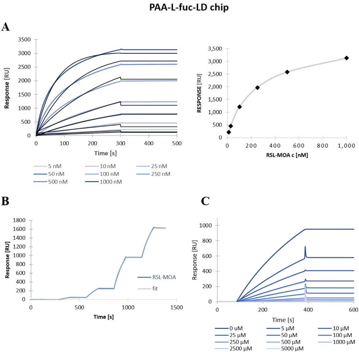
Fig. 3. SPR sensorgrams of Janus lectin RSL-MOA on CM5-PAA- \alpha -fuc LD chip. A) Titration experiment of different concentrations of RSL-MOA (blue) and fitting curves (1:1 binding fit) (black) (left) and steady-state analysis of RSL-MOA titration (right). B) Single-cycle kinetics of RSL-MOA with concentrations of 10, 50, 250, and 500 nM. C) Inhibition of 50 nM RSL-MOA by various concentration of fucose. (For interpretation of the references to color in this figure legend, the reader is referred to the web version of this article.)
