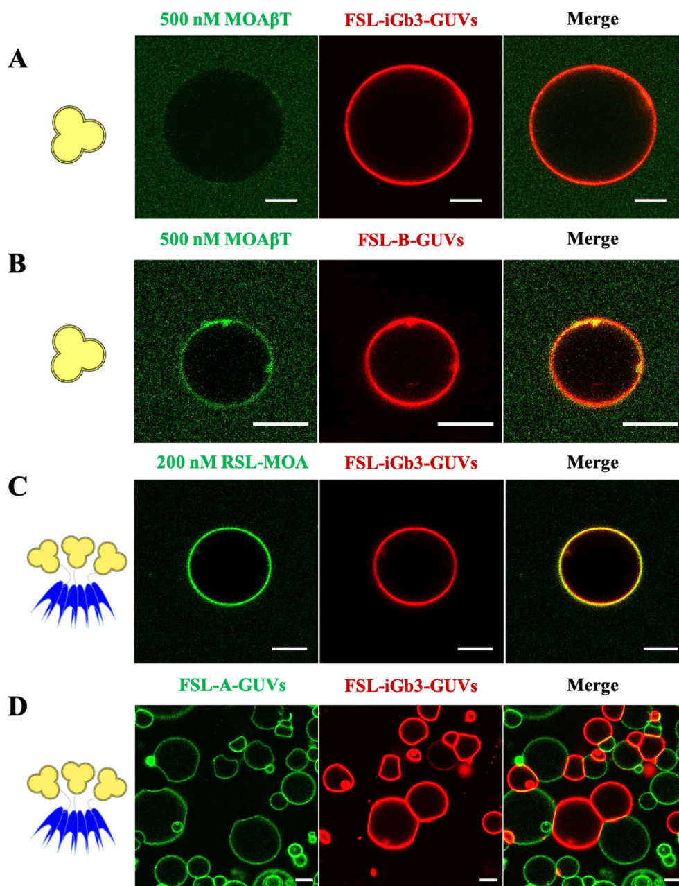
Fig. 4. The binding properties of MOAβT and RSL-MOA to glyco-decorated GUVs. A) 500 nM MOAβT-Atto488 (green) shows almost no binding to the FSL-iGb3-GUVs (red, labelled with fluorescent lipid Atto647N-DOPE). B) 500 nM MOAβT-Atto488 (green) binds to FSL-B-GUVs (red, labelled with fluorescent lipid Atto647N-DOPE). C) 200 nM RSL-MOA-Atto488 (green) binds to FSL-iGb3-GUVs (red, labelled with fluorescent lipid Atto647N-DOPE). D) Unlabeled 200 nM RSL-MOA binds two different populations GUVs FSL-iGb3-GUVs (red, labelled with fluorescent lipid Atto647N-DOPE) and FSL-A-GUVs (green, labelled with fluorescent lipid Atto488-DOPE) and crosslinks them. The GUVs were composed of DOPC, cholesterol, glycolipid of choice, and membrane dye to the proportion of 64.7:30.5:0.3 mol%, respectively. Scale bars are 10 μm. (For interpretation of the references to color in this figure legend, the reader is referred to the web version of this article.)
