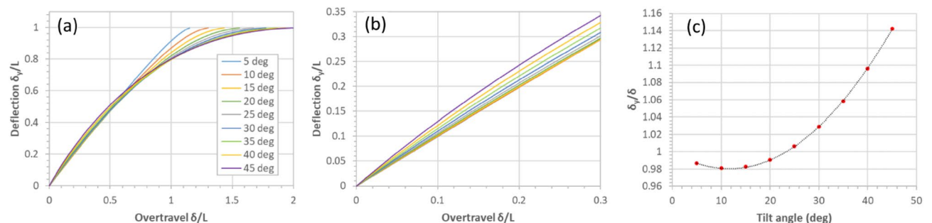
Figure 16. The relationship between overtravel and vertical deflection of the tip of a tilted triangular cantilever. (a) tip deflection as a function of imposed overtravel for various tilt angles. (b) the quasi-linear portions of the curves. (c) the tip deflection/overtravel ratio as a function of the cantilever tilt angle.
