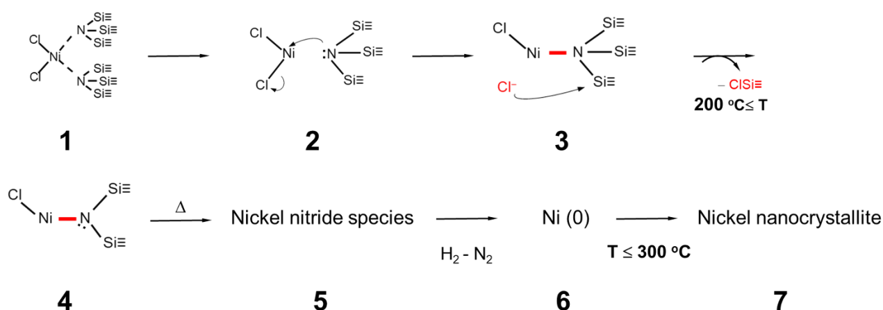
Scheme 2. Reaction scheme suggested for in situ formation of nickel nanocrystallite: Pre-formed Ni (II) complex (1) offers the nucleophilic attack of N atom of the silylamino group on the center Ni(II) cation to replace Cl (2). Subsequently, Ni-N bond formation proceeds accompanied by the attack of the released chloride anion ( \text{Cl}^- ) on other electrophiles, such as Si center of PHS moieties (3). The resulting species with a Ni-N bond (4) decompose to give nickel nitride species (a possible one is \text{Ni}_3\text{N} ) (5). Subsequent decomposition of (5) is facilitated by an in situ-formed \text{H}_2 leads to the formation of Ni (0) (6), followed by the nucleation and crystallization of Ni (7) at 200 to 300 ^{\circ}\text{C} .
