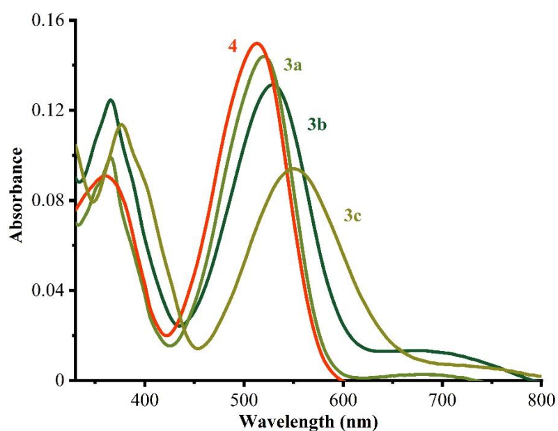
Figure 4. Absorption spectra of dyes 3a-c and 4 in DMSO solution. C = 10 \mu\text{mol}\cdot\text{L}^{-1} , l=1.00 \text{ cm}
