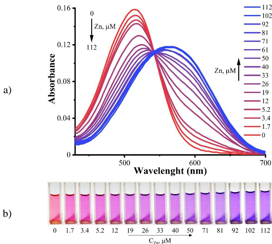
Figure 8. Absorption spectra of dye 4 without and in the presence of different amount of Zn 2+ , C_4 = 9.9 \mu\text{mol}\cdot\text{L}^{-1} , Tris-buffer (pH 7.2)/DMSO (1/3, v/v) (a); photographs of dye 4 in the presence of different amount of Zn 2+ (b); Concentration of Zn 2+ is shown in the insets.
