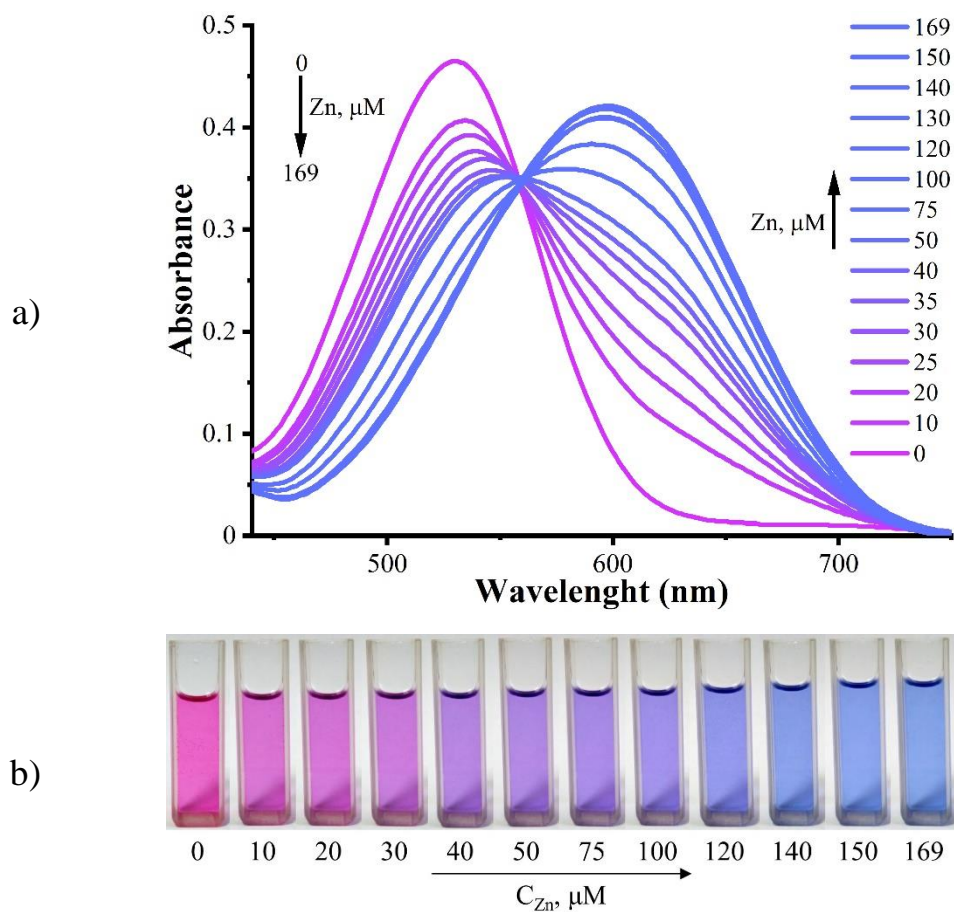
Figure 7. Absorption spectra of dye 3b without and in the presence of different amount of Zn^{2+} , C_{3b} = 38 \mu\text{mol}\cdot\text{L}^{-1} , Tris-buffer (pH 7.2)/DMSO (1/5, v/v) (a), photographs of dye 3b in the presence of different amount of Zn^{2+} (b); Concentration of Zn^{2+} is shown in the insets.
