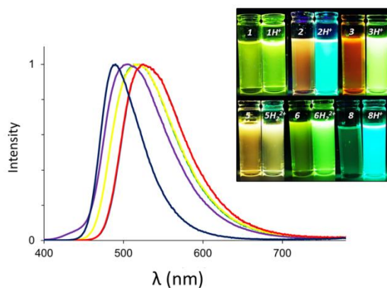
Figure 4. Emission spectra of 1 (green), 2 (yellow), 3 (purple), 5 (blue), 6 (red), 8 (navy blue) in their protonated state in dichloromethane at 25°C. (Insert) Photographs of solution in neutral (left) and protonated (right) dichloromethane under irradiation from a bench UV-lamp ( \lambda_{\text{exc}} = 365 \text{ nm} ).
