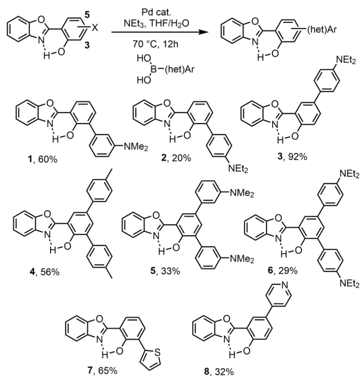
Scheme 1. Synthesis of (hetero)arylated dyes 1-8 .
