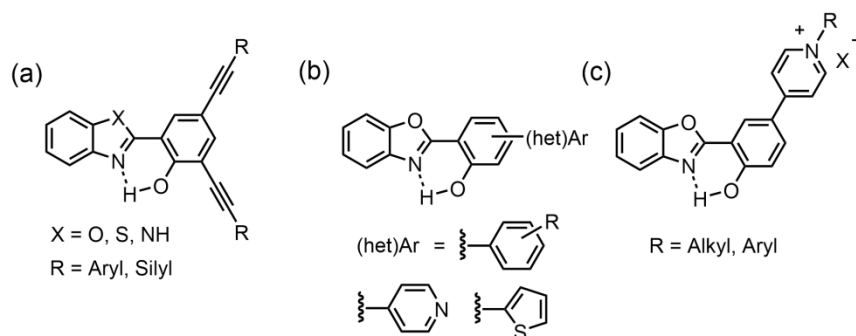
Figure 1. (a) Ethynyl-extended HBX derivatives, 13b,16-18 (b) (Hetero)arylated HBO dyes (first series) and (c) Alkyl/aryl pyridinium HBO dyes (second series) reported in this article.
