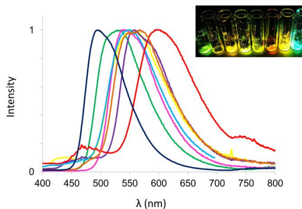
Figure 3. Emission in the solid-state, as embedded in KBr pellets (concentration of around 10^{-4} M) of 1 (green), 2 (yellow), 3 (purple), 4 (pink), 5 (blue), 6 (red), 7 (orange), and 8 (navy blue). (Insert) Photographs of solutions of dyes 1-8 as powders under irradiation from a bench UV-lamp ( \lambda_{\text{exc}} = 365 nm).
