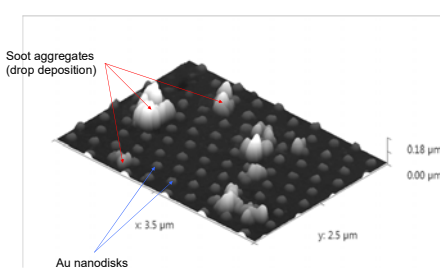
AFM image (tapping mode) - AFM PSIA XE-100
