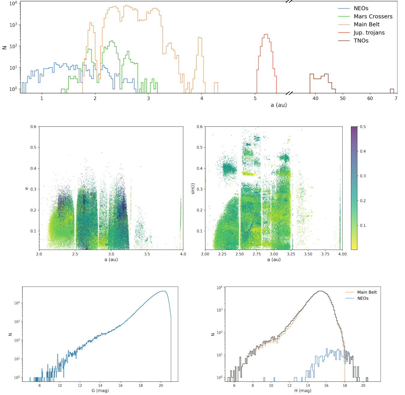
Fig. 4: Visual portfolio of some data properties for asteroids in Gaia DR3. In the top panel, we show the distribution on the semi-major axis of objects belonging to the main populations (eight Centaurs are excluded). The bin size is 1/30 au in the left part and 1/ au for TNOs. Middle panel: Distribution of main-belt asteroids in the proper elements as provided by AstDys on the a, e (left) and a, \sin(i) planes (right). Colours represent \sin(i) and e , respectively. The left bottom panel presents the distribution of the published G magnitude per transit. The cut imposed at G = 21 is visible. The right bottom panel shows that the distribution of the H magnitudes of the objects, as provided by the Minor Planet Center, is strongly dominated by main-belt asteroids, with a contribution from NEOs for the faintest sources.
