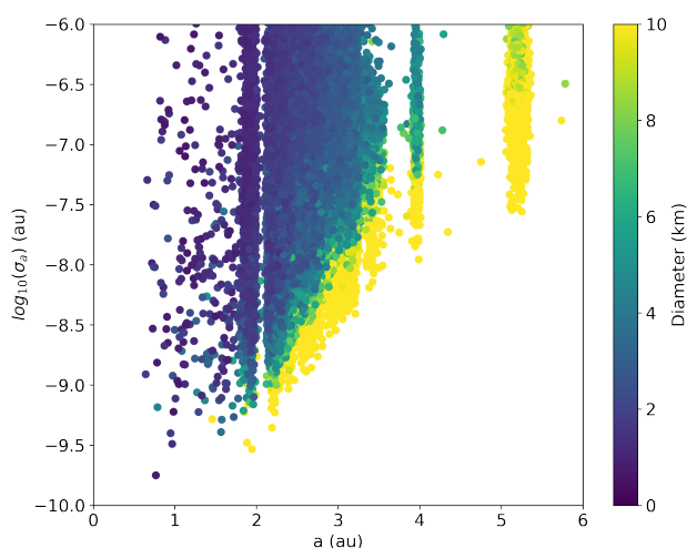
Fig. 20: Semi-major axis (au) vs log 10 of the semi-major axis uncertainty (au) for the objects for which the orbit determination procedure converged during the validation process. The colour bar represents the diameter estimate for each object from JPL SBDB.
