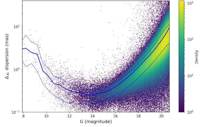
Fig. 12: Dispersion of post-fit residuals in AL for each transit. The colour represents the data density. The deep blue line shows the mean, and the light blue lines show the quantiles corresponding to 1-sigma, computed over 50 bins in the interval of G magnitude from 8 to 21 mag.
