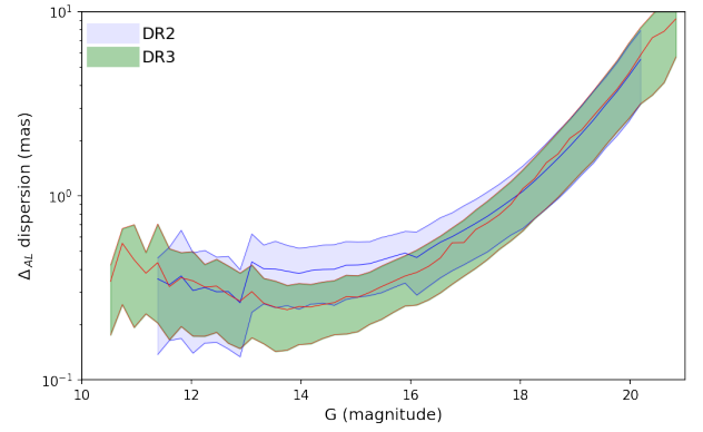
Fig. 13: Average and 1- \sigma quantiles for the AL dispersion of the post-fit residuals for all transits in common between DR2 and DR3. In contrast to Fig. 12, the single data points are not represented. The background curve (light blue) represents the distribution computed for Gaia DR2.
