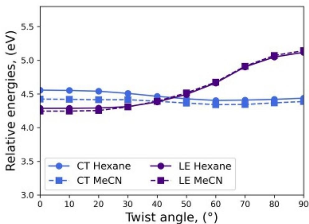
(c) PCM-BSE/evGW/B3LYP
