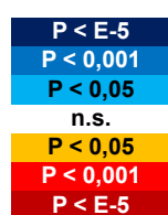
Fig. S17 Differentially expressed components of core plastid and mitochondrial metabolism in (a) ptEnolase and (b) ptPGAM1A mutants compared to empty vector control lines under 19C CL conditions, shown per Fig. S7. Cells are shaded based on DESeq P-value of gene expression difference, with blue cells indicating upregulation and red cells downregulation compared to control lines. Where more than one gene exists for an encoded function in the Phaeodactylum genome, only the most strongly differentially expressed isoform is shown.
