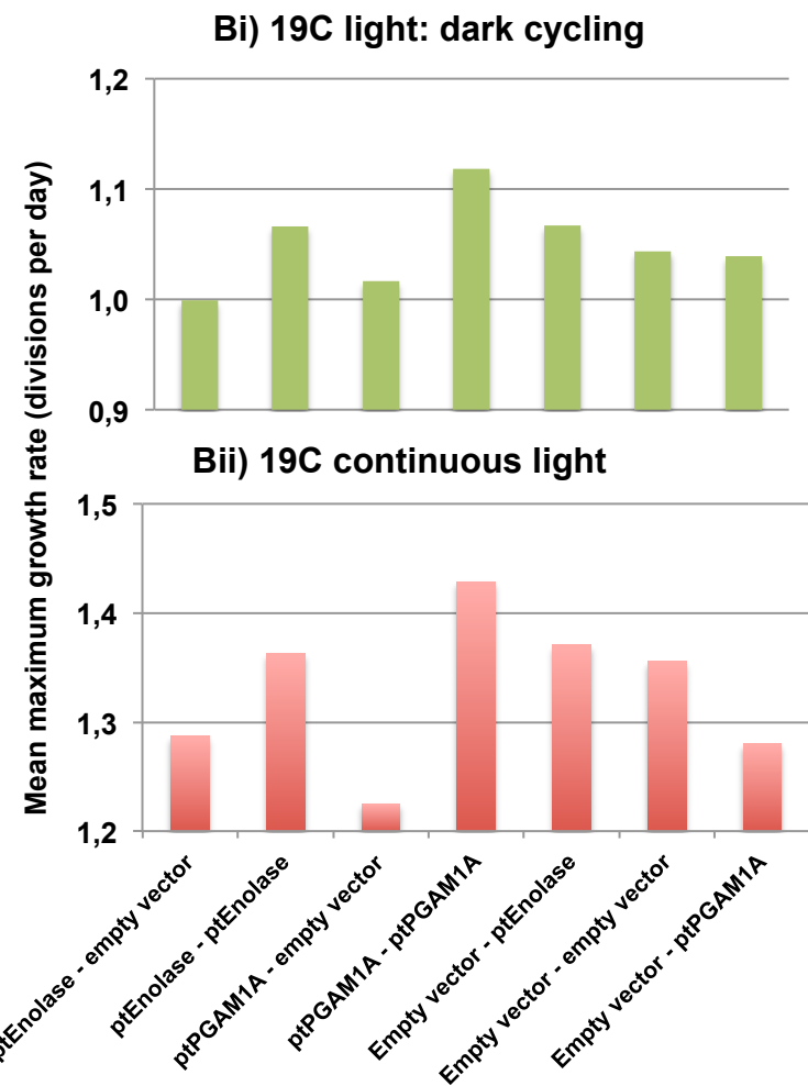
Fig. S13. Growth phenotypes of complemented glycolysis mutants. A: scatterplot of maximum growth rates, calculated from two replicates, under 19C LD cycling (horizontal) and 19C CL conditions (vertical axis) for 47 total ptEnolase (i) and ptPGAM1A mutants (ii) complemented with blasticidin-resistant and GFP-linked ptEnolase, ptPGAM1 or blank constructs, compared to empty vector zeocin-resistant control lines transformed with the same constructs. The distribution of individual growth rates within complemented and blank transformed populations are shown using solid coloured, and grey dashed line circles respectively. Vectors plot the difference between the mean growth rates calculated for blank transformed versus complemented mutant lines, alongside ANOVA P-values of separation. B: mean growth rates calculated for blank transformed and complemented mutant lines, alongside empty vector primary transformants complemented either with blank, ptEnolase or ptPGAM1A constructs, showing effective overlap between complemented mutant and empty vector primary transformant line growth rates.
