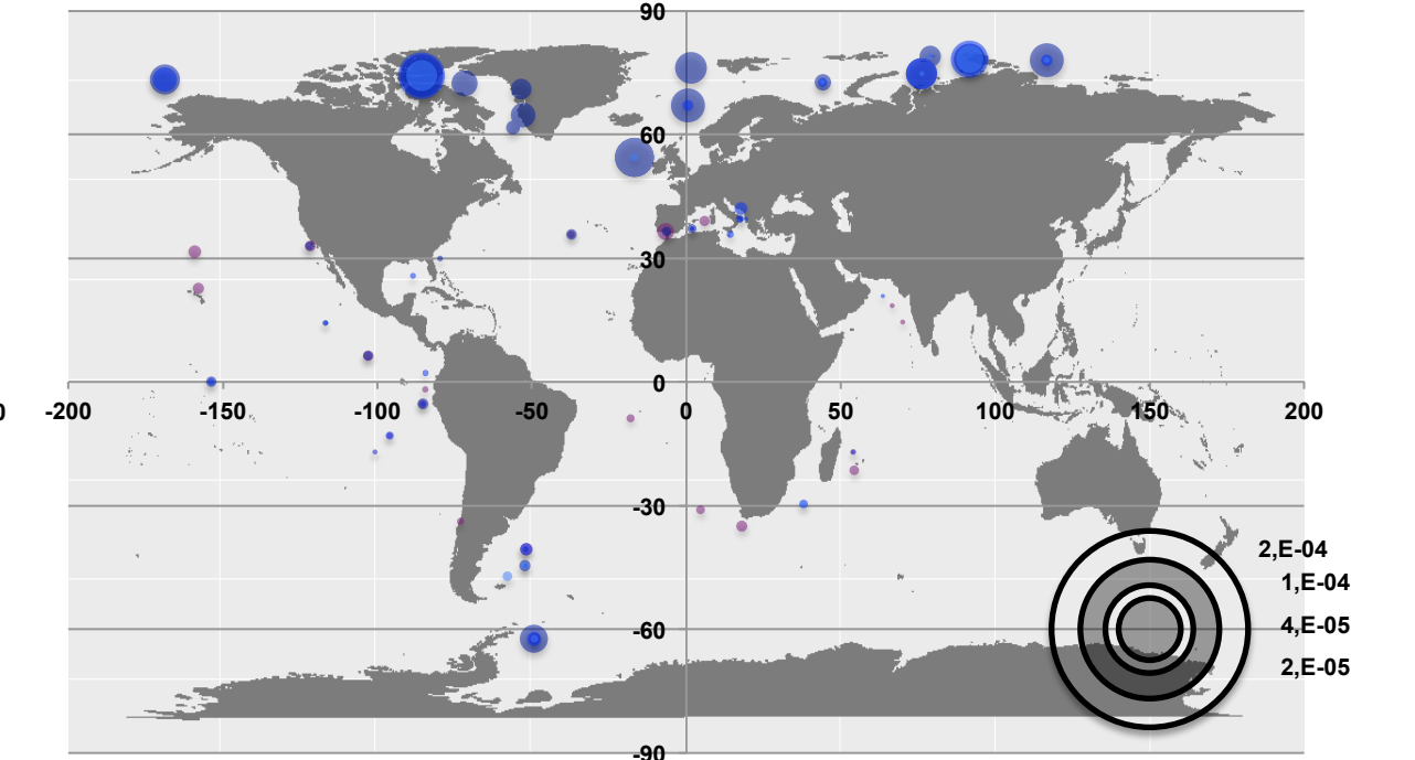
(iv) ptPGAM1 metaG abundances, DCM
