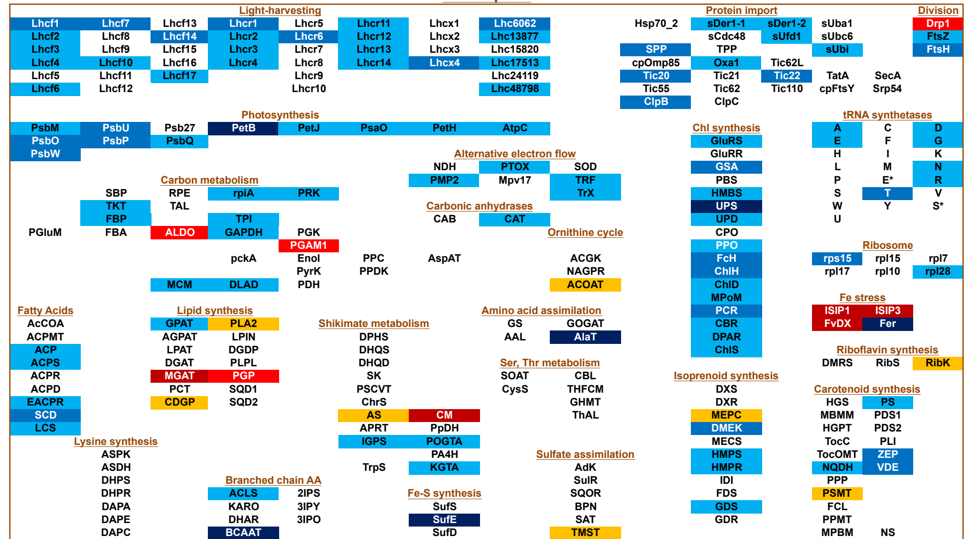
(b) ptPGAM1A mutants compared to empty vector controls DEGs, 19C CL conditions
