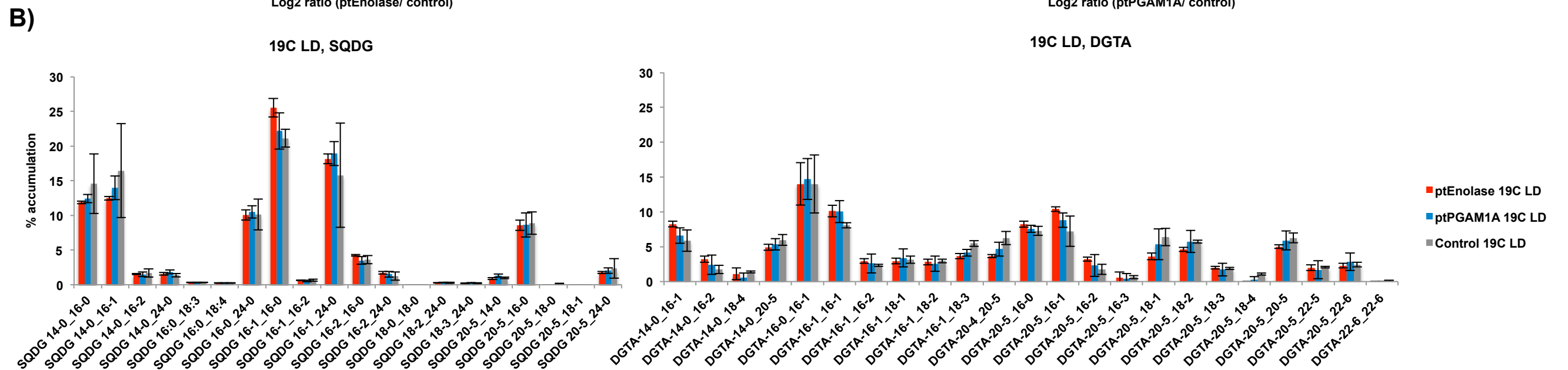
Fig. S20. Differentially accumulated lipids in 19C LD condition. A: Volcano plots shows (horizontal axis) \log_2 accumulation ratios and (vertical axis) -\log_{10} ANOVA Pvalues for separation of mean proportions of specific fatty acids, across all fatty acids observed in a specific lipid class in glycolysis mutants versus control lines, harvested under 19C LD conditions. Specific lipids that show extreme ( P < 10^{-05} ) differences in accumulation between both mutant genotypes and control lines are labelled, and coloured by lipid class. B: Bar plots showing total DGTA lipid class distributions in all three lines under these conditions. These data suggest limited changes in glycolysis mutant lipid architecture, barring a probable overaccumulation of sn -1 C16 in ptEnolase mutant MGDG and DGDG pools, a corresponding underaccumulation of sn -1 C20 in ptEnolase mutant DGTA pools, and a conserved underaccumulation of DGTA-16-1_18-3 in both ptEnolase and ptPGAM1A mutants.
