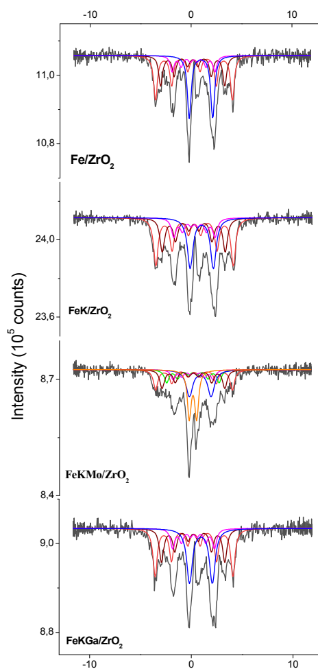
Figure 11. Mössbauer spectra after activation measured at -153 °C.
