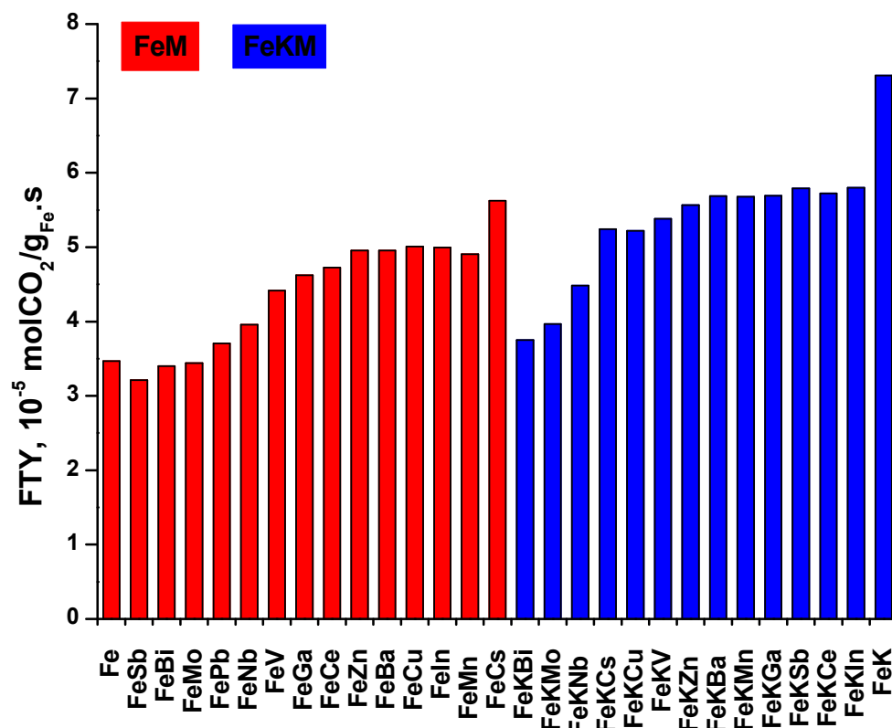
Figure 1. Carbon dioxide conversions and iron time yields (FTY) measured over the promoted zirconia supported iron catalysts T=350\text{ }^{\circ}\text{C} , \text{H}_2/\text{CO}=3 , p=10\text{ bar} , TOS = 50 h.
