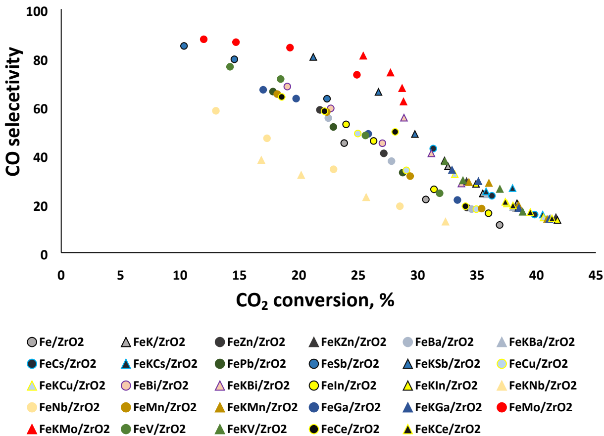
Figure 2. CO selectivity versus carbon dioxide conversion for the Fe/ZrO 2 promoted catalysts. T=350°C, H 2 /CO=3, WHSV=4.67-18.19 L/ g.h, P=10 bar, TOS = 50 h.
