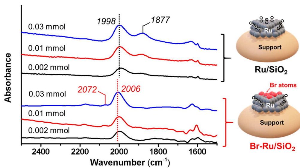
Figure 5. CO-FTIR for Ru/SiO 2 and Br-Ru/SiO 2
