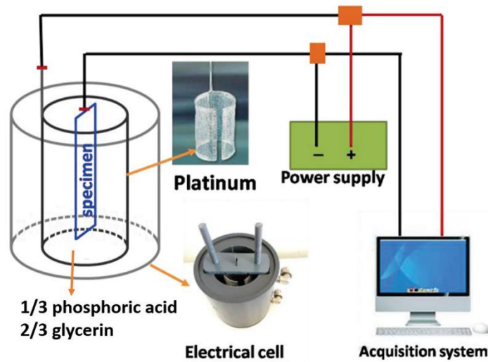
Fig. 1 Schematic presentation of the hydrogen charging system [25]
