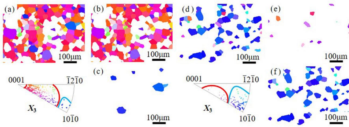
Fig. 3 (a) IPF map of initial Group I grains and corresponding IPF on Surface A (b) IPF map of initial B-type grains on Surface A (c) IPF map of initial P-type grains on Surface A (d) IPF map of initial Group I grains and corresponding IPF on Surface B (e) IPF map of initial B-type grains on Surface B (f) IPF map of initial P-type grains on Surface B
