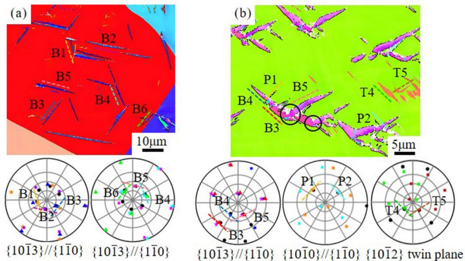
Fig. 10 IPF maps of Group II grains with hydride platelets and corresponding pole figures of hydride interface planes and twin planes (a) Grain 4, Euler angle: 155.2, 6.4, 43.3 (b) Grain 5, Euler angle: 175.0, 120.5, 58.5. In (b), the blue curves represent the boundaries between two hydride variants. In the pole figures of hydride interface planes, the black dots represent the \{10\bar{1}3\} or \{10\bar{1}0\} interface planes of Ti matrix and the colors represent the \{1\bar{1}0\} interface planes of hydrides. In the pole figures of twin planes, the black dots represent the \{10\bar{1}2\} twin planes in the matrix and the colors represent the twin planes in twins. The dotted line represents the trace of the corresponding hydride interface planes and twin planes.
