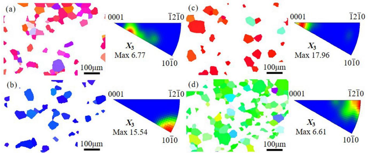
Fig. 4 IPF map of initial grains and corresponding IPF. (a) Grains forming full-covered B-type hydride layer after hydrogen charging (b) Grains forming full-covered P-type hydride layer after hydrogen charging (c) Grains which are non-indexed after hydrogen charging (d) Grains forming few hydrides after hydrogen charging
