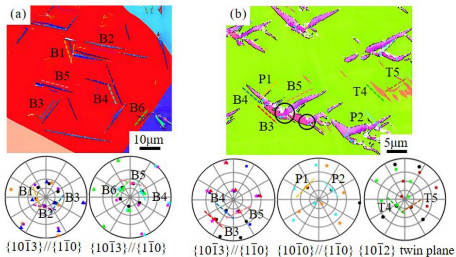
Fig. 10 IPF maps of Group II grains with hydride platelets and corresponding pole figures of hydride interface planes and twin planes (a) Grain 4, Euler angle: 155.2, 6.4, 43.3 (b) Grain 5, Euler angle: 175.0, 120.5, 58.5. In (b), the blue curves represent the boundaries between two hydride variants. In the pole figures of hydride interface planes, the black dots represent the \{10\bar{1}3\} or \{10\bar{1}0\} interface planes of Ti matrix and the colors represent the \{1\bar{1}0\} interface planes of hydrides. In the pole figures of twin planes, the black dots represent the \{10\bar{1}2\} twin planes in the matrix and the colors represent the twin planes in twins. The dotted line represents the trace of the corresponding hydride interface planes and twin planes.
