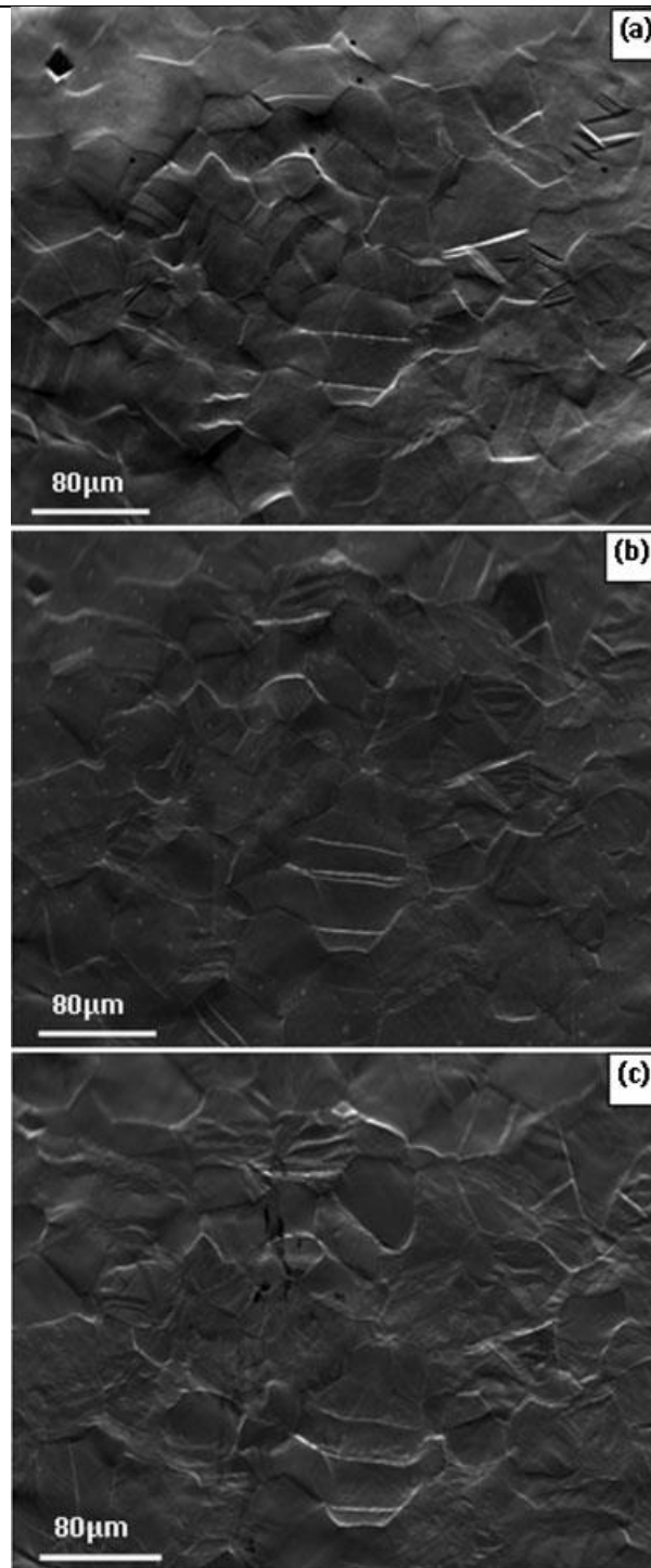
Fig. 2 Field emission gun SEM microstructure of a 10%, b 20% and c 30% deformed sample
