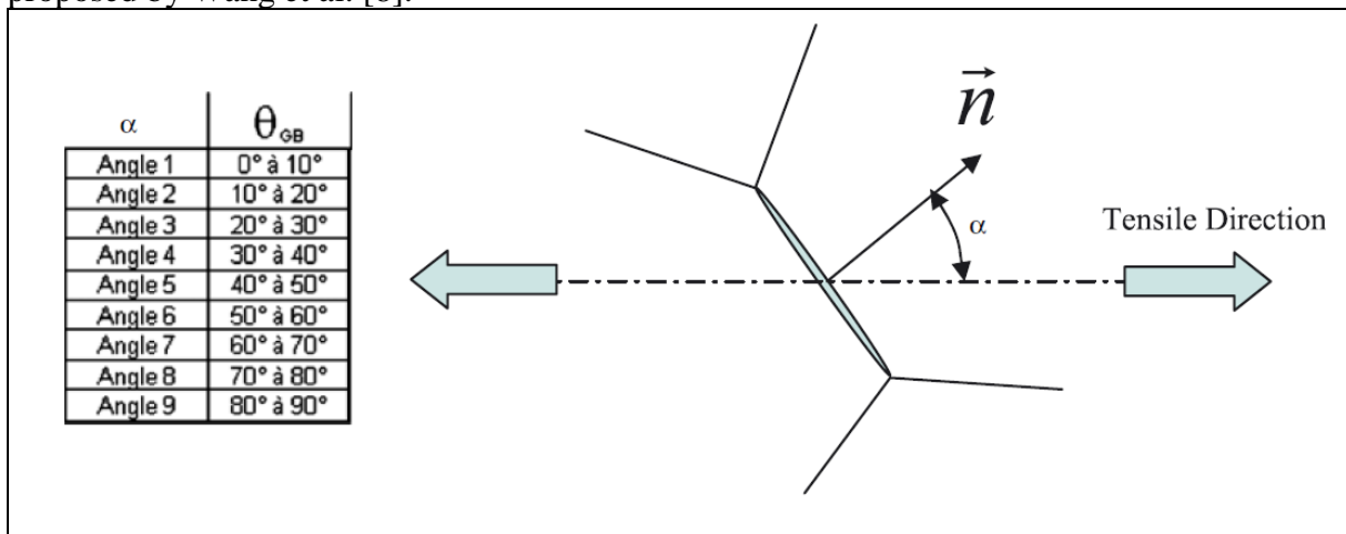
Fig. 9 Orientation of the grain boundary plane with respect to the uniaxial tensile direction. Nine angle classes \alpha were defined from 10° to 10° in the angular range from 0° to 90°
