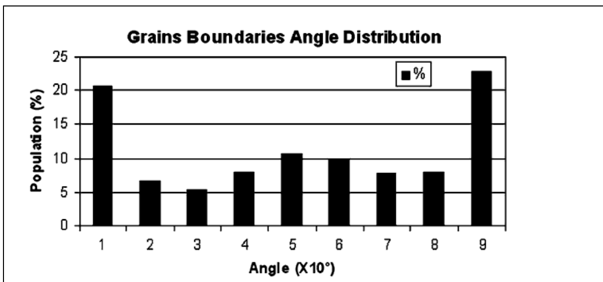
Fig. 10 Distribution of the grain boundary orientations according to the angle \alpha defined by the normal to the grain boundary plane and the direction of uniaxial tension
