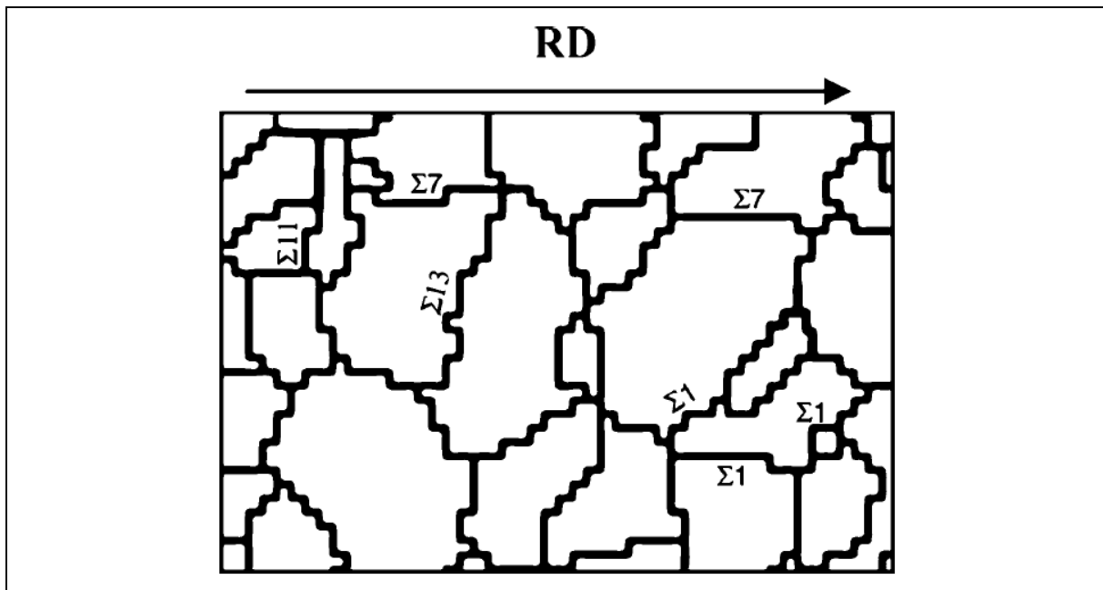
Fig. 5 OIM micrograph of the hot-dip galvanized zinc coating. Coincident boundaries ( S \leq 28 ) are selected according to the Brandon-type criterion (Eq. 1) with m_0 = 10^\circ . Non-labeled boundaries are random grain boundaries
