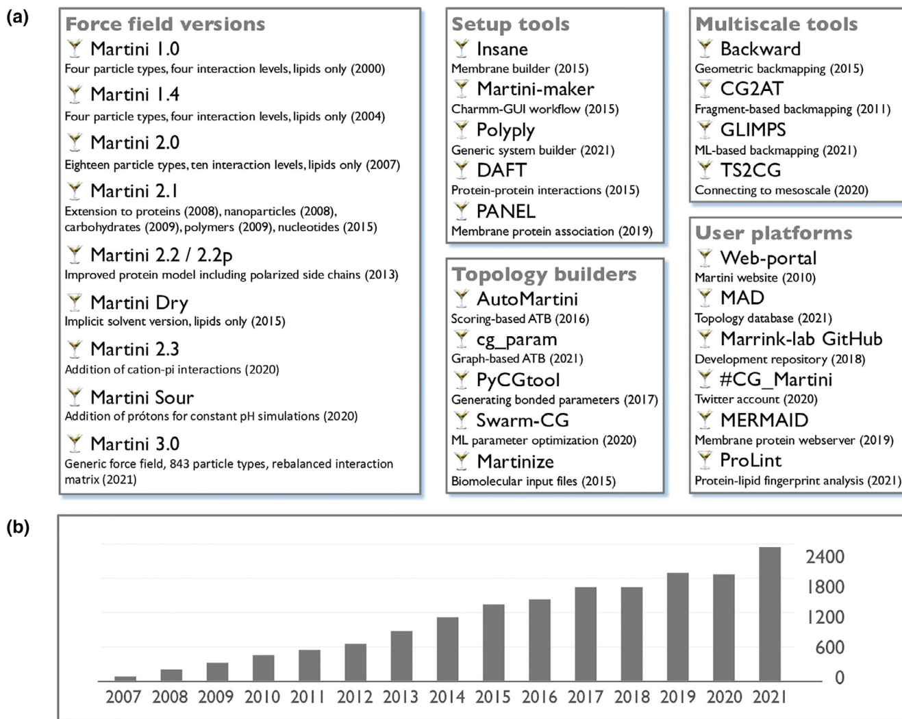
FIGURE 1 Historical overview of the Martindome. (a) The different force field versions are listed in the leftmost box, a selection of popular auxiliary tools for the setup of starting structures, building of topologies, converting to other resolutions, and user platforms are shown in the other boxes. (b) Growing citation numbers for the basic Martini papers, taken from the Martini google scholar profile. 26
