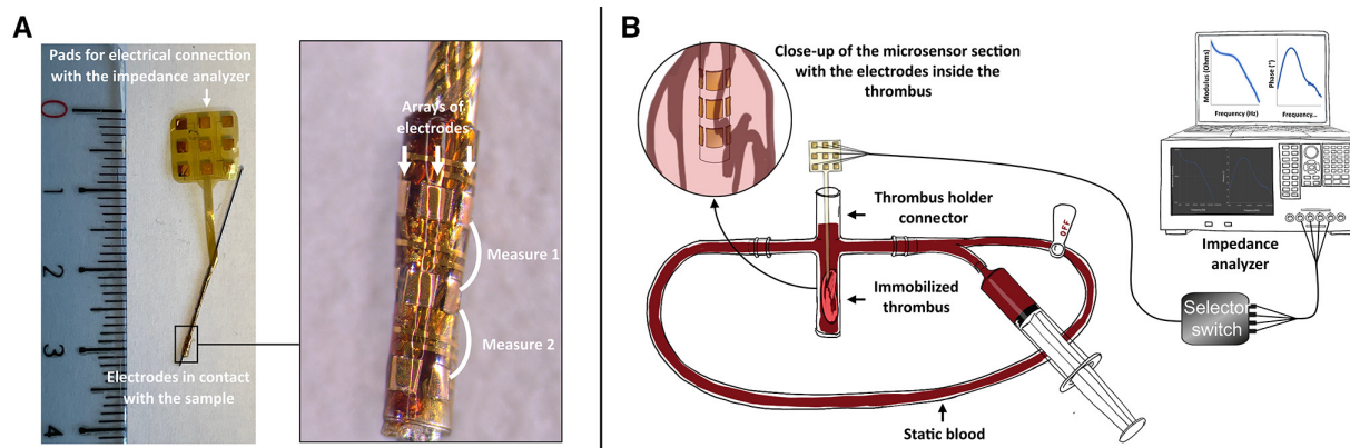
Figure 1 (A) Custom-made in vitro polyimide flexible device rolled over a 300 μm diameter metal wire (diameter comparable to a 0.014 inch neurovascular guidewire). The close-up shows the electrodes and indicates between which electrodes the measurement is performed. (B) Experimental setup. A custom-made microsensor was inserted in a thrombus holder filled with blood to mimic the environment of a large-vessel occlusion. For the measurement, the microsensor was inserted either in blood or in the thrombus while measurements were taken with the impedance analyzer. A custom-made selector switch allowed multiple measurements to be made on adjacent pairs of electrodes along each of the three rows of electrodes. Custom-made software is used to control the impedance analyzer.
