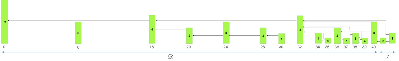
(b) View of the blockchain after compression at time t .
