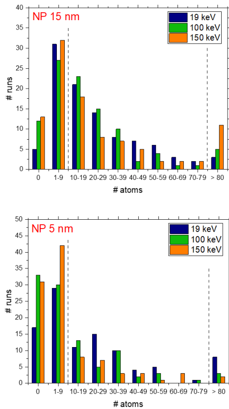
Figure 8- Number of sputtered atoms for a 5 nm NP (lower case) and for a 15 nm NP (upper case). Zero means that only the PKA escapes the NP (no sputtering). Total number of runs = 100.
