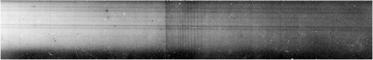
Figure 18: Lower panel: the solar spectrum obtained at Mont Blanc with the Rowland grating spectrograph. The B band of oxygen spectral lines ( O_2 molecule) appears at the wavelength of 680 nm, in the red. Upper panel: the spectrum of the Jungfrauoch (3600 m) for comparison, degraded to almost the same resolution and observed by Delbouille et al (1973) with wavelength indicated in Angström (courtesy Paris Observatory).
