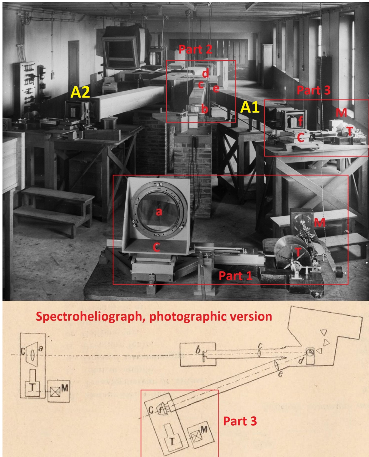
Fig. B.1. Meudon spectroheliograph in 1919. Part 1: entrance with a = imaging objective (250 mm diameter, f = 4000 mm, F/16); C = moving support; T = velocity reducer; M = motor. Part 2: spectrograph with b = entrance slit; c = collimator ( f = 1300 mm); d = prisms or grating (300 grooves/mm, 17^\circ blaze angle); e = camera lens ( f = 3000 mm). Part 3: exit with f = selective slit in the spectrum; C = moving support of photographic plates; T = speed reducer; M = motor. Arms A1 and A2 were used respectively for H\alpha (Rowland grating) and CaII K (prisms) until 1988. After this date, arm A1 was used for both (new grating). In 2002 and 2018, part 3 was successively replaced by two generations of electronic sensors (CCD, sCMOS) fed by new camera lenses (respectively 900 mm and 400 mm focal length).
