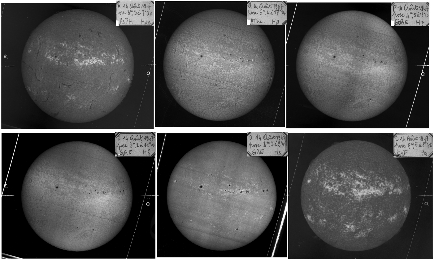
Fig. B.10. Exceptional observations of Meudon spectroheliograph, 14 August 1947. Top: the Balmer series, H\alpha , H\beta , H\gamma . Bottom: H\delta , H\epsilon (in the red wing of CaII H line) and the classical CaII K3.
