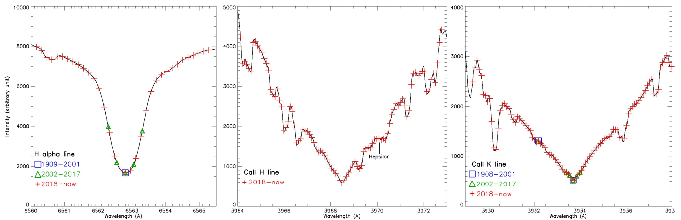
Fig. B.14. The spectra sampling in the successive versions of Meudon spectroheliograph. Left: H \alpha ; middle: CaII H (since 2018); right: CaII K. Blue squares: observed wavelengths from 1908 to 2001 (photographic plates and films). Green triangles: CCD version from 2002 to 2017. Red crosses: sCMOS version starting in 2018. Black: atlas profiles (Delbouille et al., 1973) degraded at the spectroheliograph resolution (disk centre).
