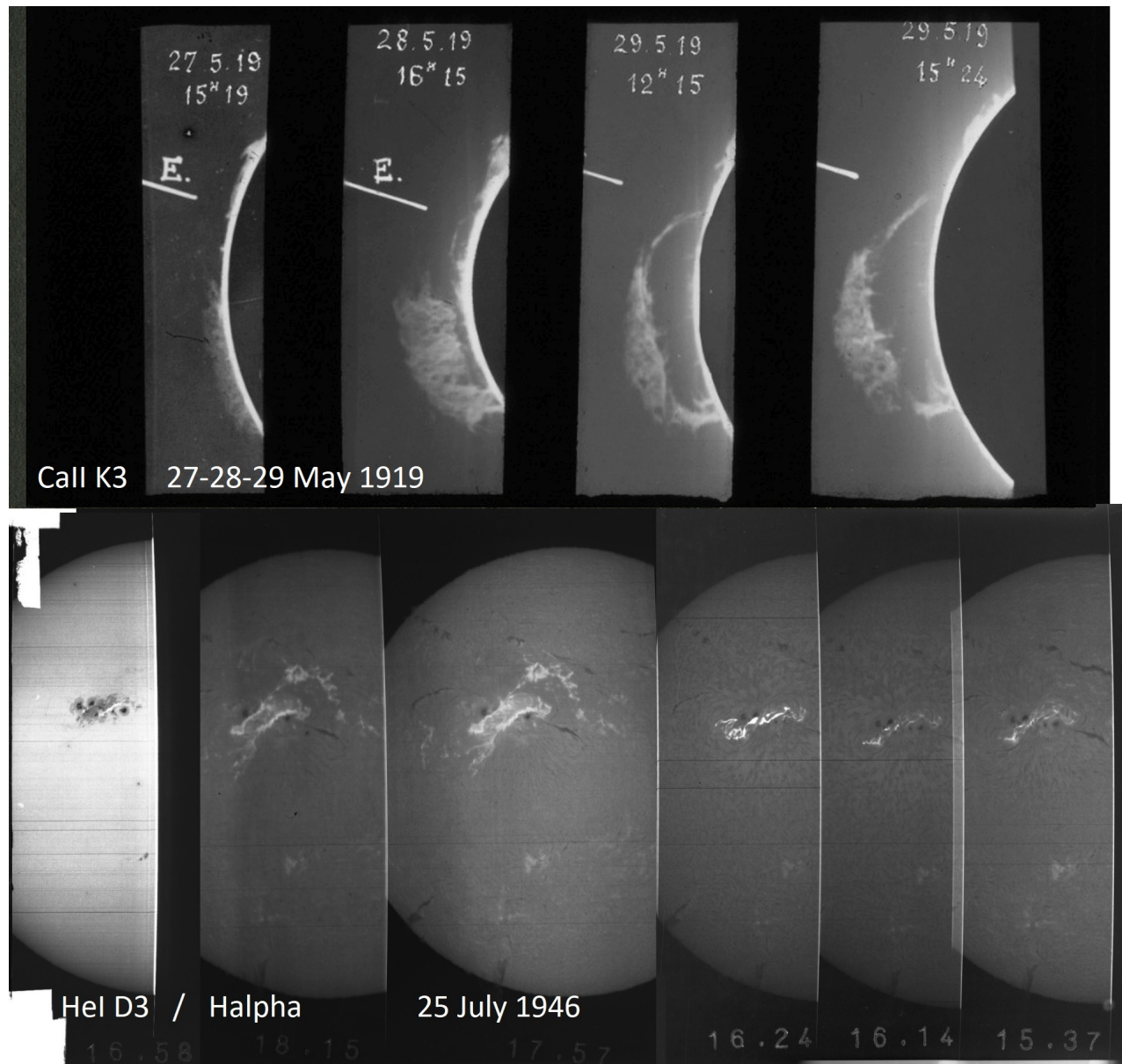
Fig. B.9. Examples of rare dynamic events observed with Meudon spectroheliograph. Top: the eruptive prominence of 27-28-29 May 1919 observed in CaII K3. Bottom: the large solar flare of 25 July 1946 observed in HeI D3 (left panel at 16:58 UT) and in H \alpha line centre at 18:15, 17:57, 16:24, 16:14 and 15:37 UT (right panels).
