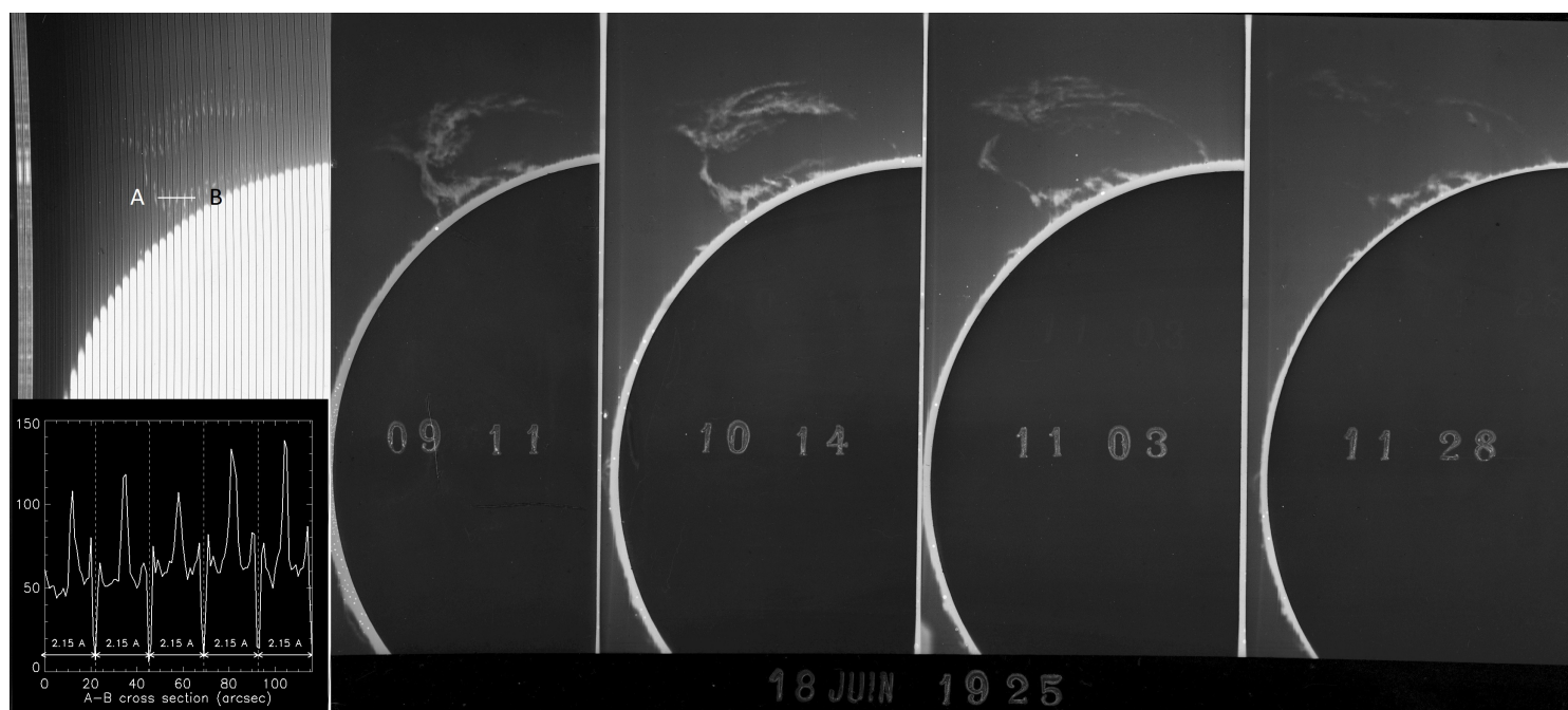
Fig. B.12. Another example of the CaII K "radial velocity" collection, the eruptive prominence of 18 June 1925. The left panel shows spectra recorded by 22 arcsec steps ( 2.15 \text{ \AA} spectral range, the disk is saturated). The five emission profiles along the cross section A-B are displayed at bottom. The other panels are the usual CaII K3 spectroheliograms recorded at 09:11, 10:14, 11:03 and 11:28 UT with an artificial moon.
