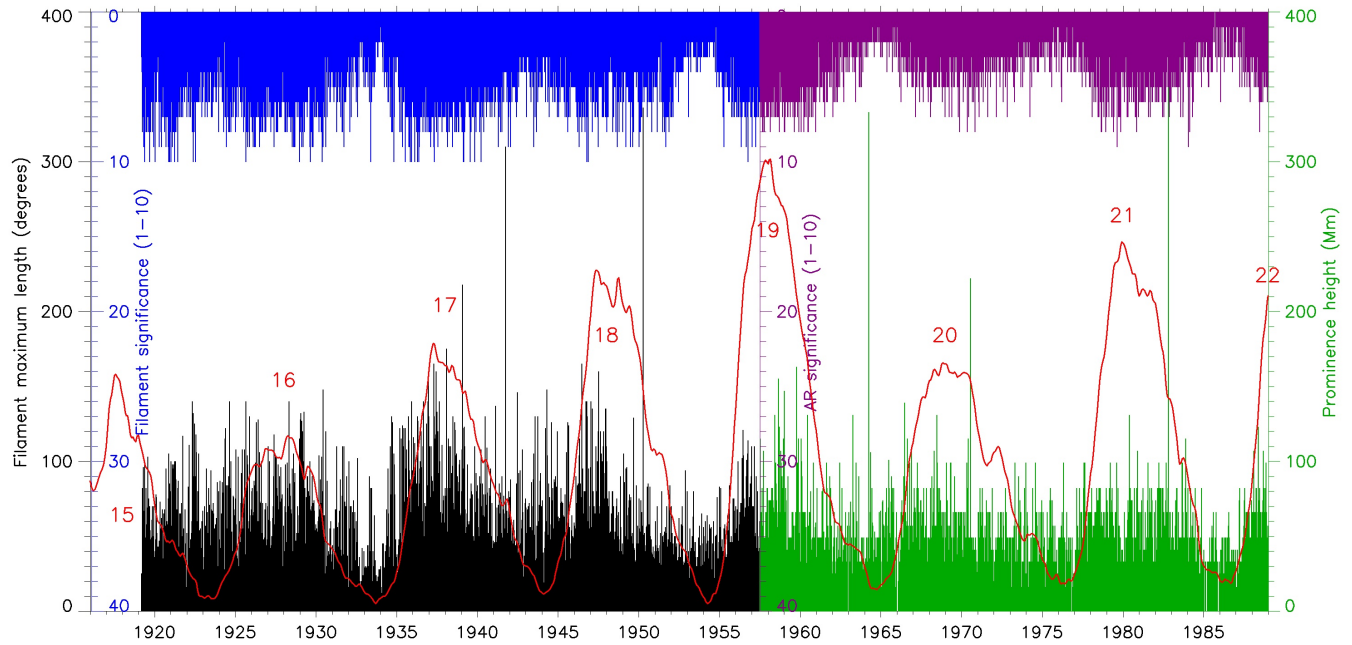
Fig. B.5. Examples of data provided by the tables associated with each Carrington rotation. Black: maximum length of filaments (degrees). Green: maximum height of prominences (Mm). Blue: filament significance (1-10 scale). Violet: active region significance (this index, in the range 1-10, is evaluated from the lifetime, the intensity and the area of facular plages, or the number and the area of sunspots). The Brussels sunspot number has been superimposed in red together with the identification of cycles.
