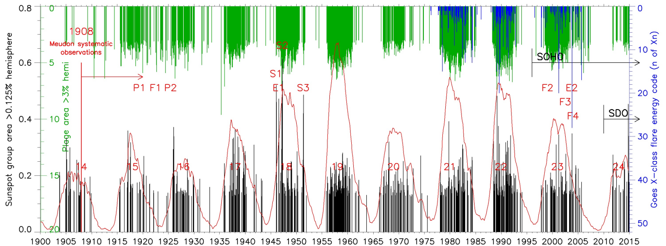
Fig. B.6. Some rare events distribution. Black: sunspot group area above 0.125% of the solar hemisphere (after Mandal et al. (2020)). Green: plage area above 3% of the hemisphere (after Chatzistergos et al. (2020)). Blue: X-class flares (X1 to X28 range). The Brussels sunspot number has been superimposed in red together with identification of cycles. P1, P2 = prominence eruptions of Figures B.9 and B.12. F1, F2, F3, F4 = long filaments of Figure B.8. E1, E2 = strong flares of Figures B.9 and B.3. S1, S2, S3 = huge sunspot groups of Figures B.7. The most significant sunspot groups were seen during cycle 18.
