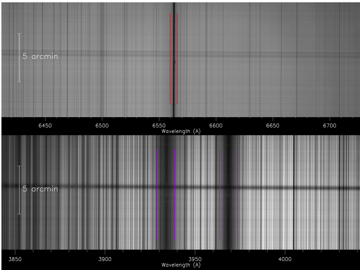
Fig. B.13. The spectral domains selected by the standard observing procedure of the 2018 version of Meudon spectroheliograph. Top: H \alpha , 6.2 Å spectral range, 0.155 Å/pixel (40 pixels). Bottom: CaII H and CaII K, 9.3 Å spectral range, 0.093 Å/pixel (100 pixels). Spectral ranges can be enlarged upon request with no impact on the recording time (just bigger files). A sunspot is present in the FOV.
