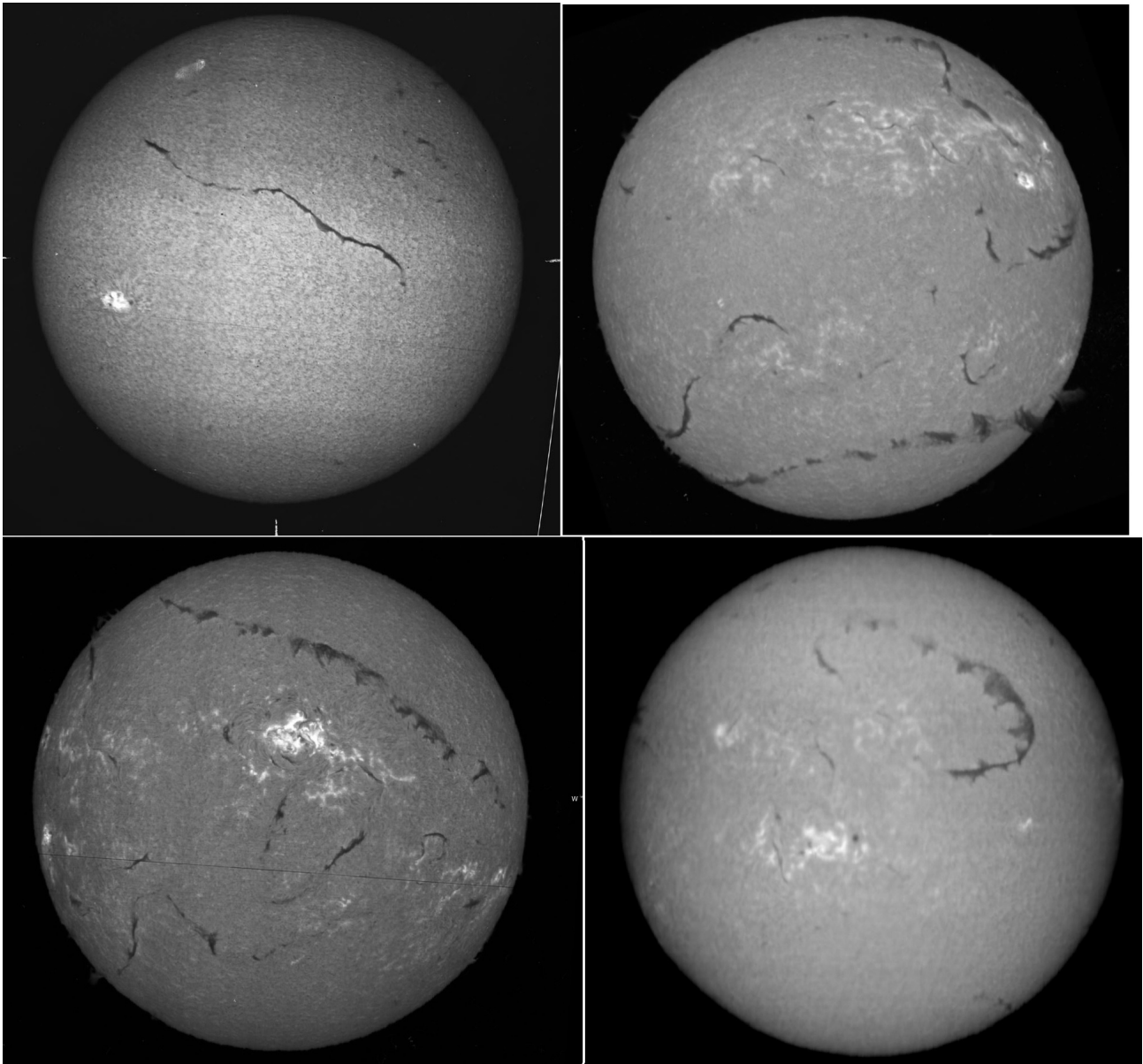
Fig. B.8. Some examples of the longest filaments observed with Meudon spectroheliograph in H\alpha centre. Top: 20 July 1922 (left) and 30 January 1999 (right). Bottom: 16 July 2002 (left) and 18 January 2004 (right).
