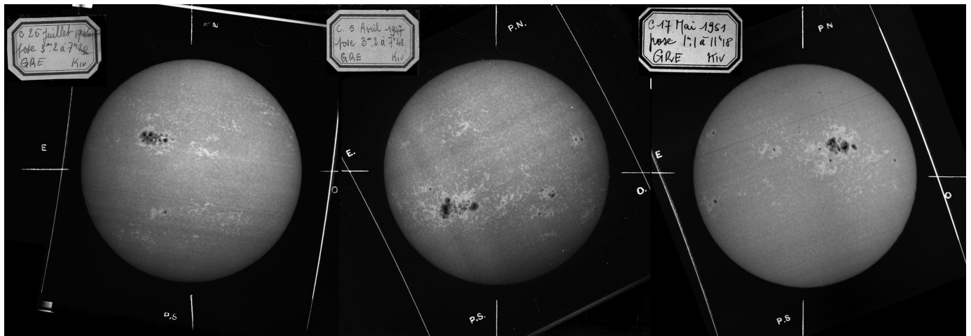
Fig. B.7. Some examples of the huge sunspot groups of cycle 18 (CaII K1v spectroheliograms): from left to right, 25 July 1946, 5 April 1947, 17 May 1951, covering respectively 0.46%, 0.61% and 0.48% of the disk area.
