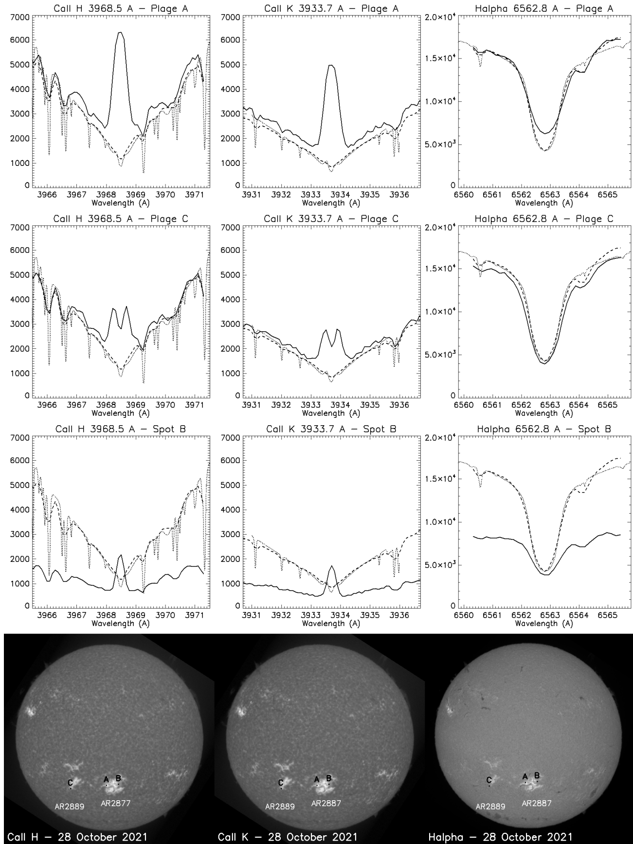
Fig. B.15. Example of line profiles provided by the 2018 version (from 3D FITS files of 28 October 2021). Column 1: CaII H (13:04 UT); column 2: CaII K (13:04 UT); column 3: H \alpha (13:01 UT). Row 1: bright plage A of AR2887; row 2: plage C of AR2889; row 3: sunspot B of AR2887; row 4: CaII H, CaII K and H \alpha images at line centre, just before the X1.0 flare at 15:35 UT in AR2887 (southern hemisphere). Solid line: line profiles of points A, B, C; dashed line: profile of disk centre; dotted line: high resolution atlas profile of disk centre (Delbouille et al., 1973).
