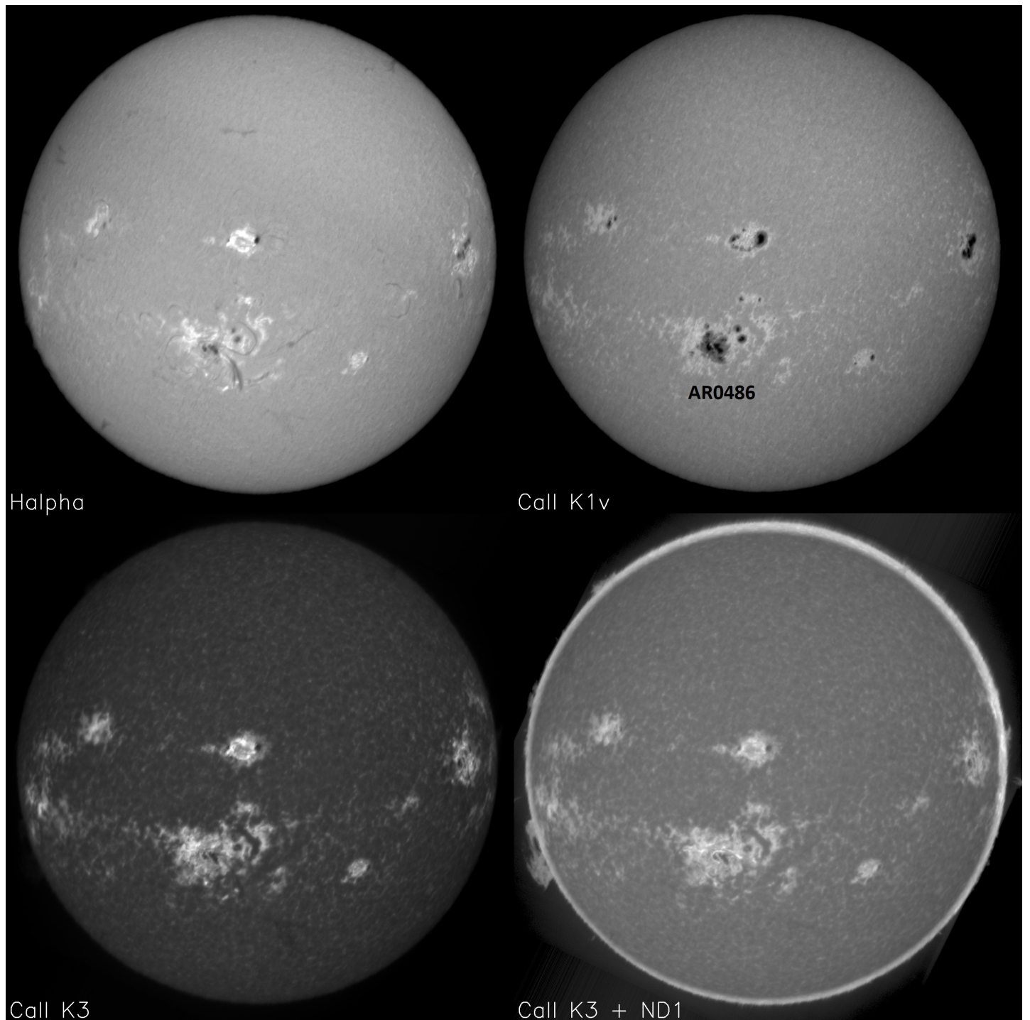
Fig. B.3. Typical images obtained daily at Meudon spectroheliograph. Example of 28 October 2003, a couple of hours before the historic X17.2 flare (11:10 UT) in the big AR0486 of the southern hemisphere. A set of spectroheliograms is composed of H\alpha centre (08:09 UT), CaII K1v (violet wing at -1.5 \text{ \AA} , 08:13 UT), CaII K3 (line centre, 08:13 UT) and a long exposure CaII K3 with the ND1 artificial moon (08:50 UT) in order to register both prominences and the solar disk.
