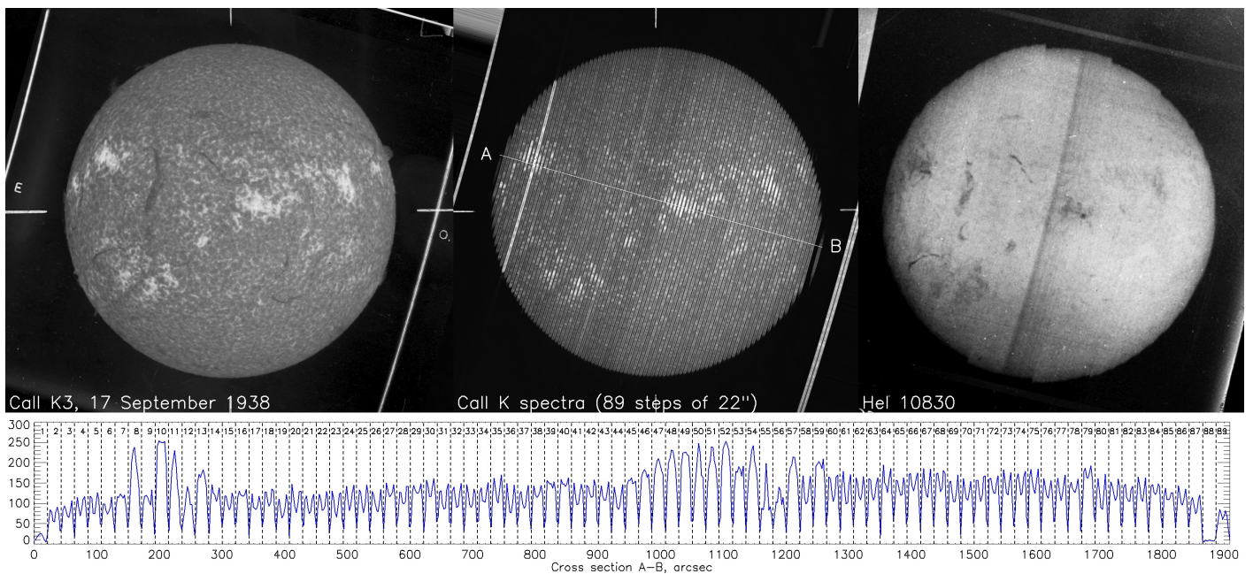
Fig. B.11. Example of the CaII K "radial velocity" collection, 17 September 1938, showing spectra recorded with a 22 arcsec step. Such spectra-images were frequently obtained from 19 April 1909 to 3 November 1943. Top: the classical CaII K3 spectroheliogram, the "radial velocity" scan of 89 slit positions across the solar disk, and the first spectroheliogram obtained worldwide in the infrared HeI 10830 Å line. Bottom: the cross section A-B shows the CaII K spectral line, step by step, for the 89 positions. The spectral range is 2.15 Å.
