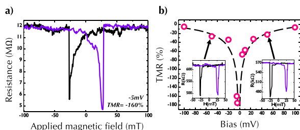
Figure 4. Spin-transport characterizations in the multilayer Ni(111)/MLGr based spin valve making use of the top \text{Al}_2\text{O}_3/\text{Co} spin analyzer. (a) Magneto-resistance signal measured at 2 K and under -5 mV DC bias in the nanojunction. The negative TMR observed of \sim 160\% comes from the efficient spin filtering effect occurring at the Ni(111)/Gr interface and leads to an extracted large negative spin polarization up to P_{\text{Ni/Gr}} = -98\% . (b) TMR dependency with respect to the DC bias applied in the junction with pink circles being experimental TMR measured at different biases (black dashed line is a guide-to-the-eye). We observe only a simple monotonous dependence of the TMR spin signal with bias, classically ascribed to FM magnons (see refs 52 and 53). Inset: two TMR measured at + and -50 mV.
