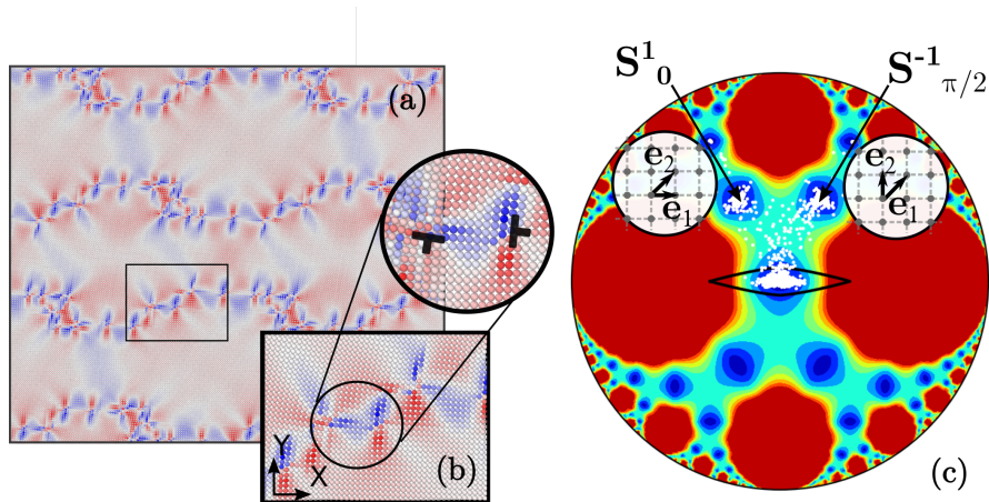
Figure 11: (a) Post-instability pattern for the rhombic path \mathbf{F}_0 , colors show the level of the Cauchy stress \sigma_{xy} . (b) Inset highlights the presence of both vertical and horizontal dislocations. (c) Distribution of \mathbf{C}_i points in configuration space show the dominant presence of the three wells \mathbf{S} , \mathbf{S}_0^1 and \mathbf{S}_{\pi/2}^{-1} . The elements on the low energy valleys connecting wells corresponds to dislocation cores.
