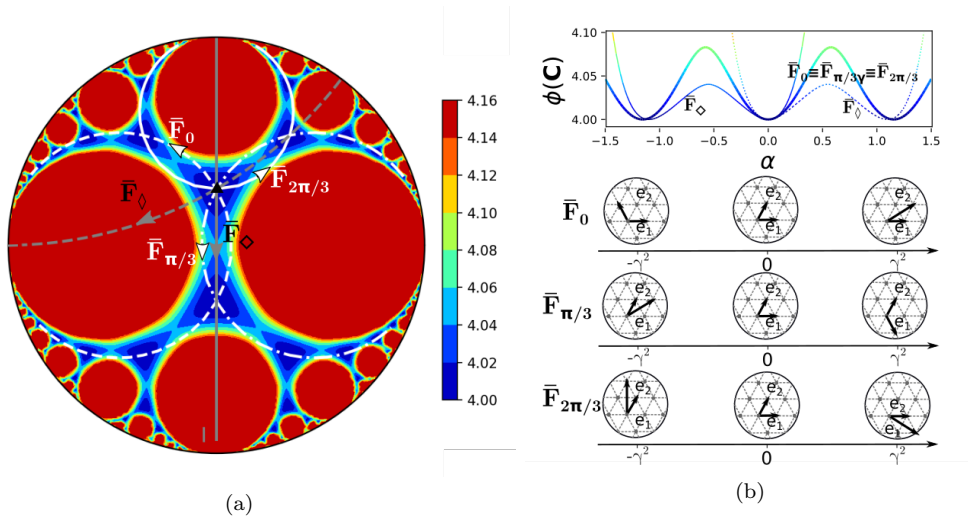
Figure 3: (a) Poincaré disk showing the energy landscape for the case \beta = 4 . Minima of the energy are located on triangular lattice configurations and simple shears form circular trajectories (shown in white). The loading paths \mathbf{F}_\diamond and \bar{\mathbf{F}}_\diamond are illustrated in grey (with a continuous and a dashed line respectively). (b) Energy landscape along shearing deformation paths \bar{\mathbf{F}}(\alpha, 0) , \bar{\mathbf{F}}(\alpha, \pi/3) and \bar{\mathbf{F}}(\alpha, 2\pi/3) , the shear-invariant triangular configurations are illustrated below the corresponding energy wells. The non-symmetric energy landscapes along the two pure shear paths are shown as well for comparison.
