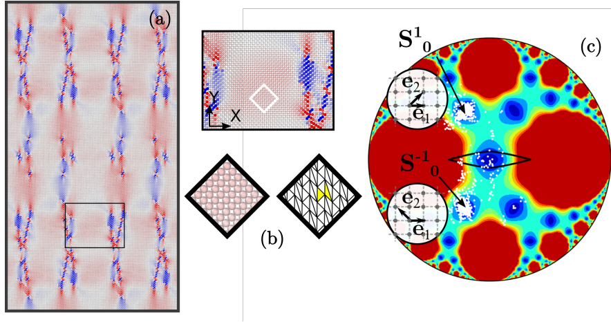
Figure 13: (a) Post-instability pattern for the rectangular path \mathbf{F}_\square , colors indicate the level of the Cauchy stress \sigma_{xy} . (b) The insets allow one to visualize the \pi/4 rotated structure, the triangulation reveals the shearing mechanism behind such apparent rotation. (c) Distribution of C_i points in configuration space show the splitting of the system between the wells \mathbf{R}^{\pi/4}\mathbf{S}_1^0 and \mathbf{R}^{-\pi/4}\mathbf{S}_{-1}^0 .
