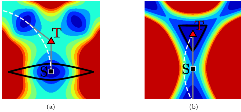
Figure 6: (a) Stability (yielding) limits for the square crystal (in black). The two loading paths corresponding to simple shear \mathbf{F}_0 (dashed white) and rhombic pure shear \mathbf{F}_{\circ} (grey) cross the stability region in similar configurations. (b) Stability region for the triangular symmetry crystal (black). Here the difference of strain configurations at the limit of stability is larger if we compare the loading paths corresponding to simple shear (dashed white) and pure shear (grey).
