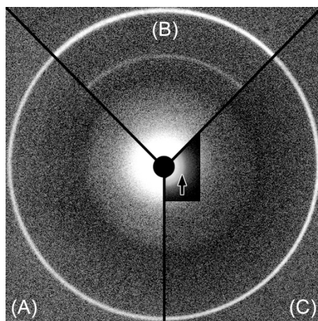
Figure S4. Comparison of the low-angle XRD powder patterns (laboratory set-up) of hydrated V8 II complexes prepared by crystallizing amylose in the presence of naphth-1-ol (A – DP130), salicylic acid (B – DP80) and quinoline (C – DP2500), focusing on a 2\theta region extending to 2\theta = 9^\circ . By comparison with the patterns shown in Figure 2C,F,I , the sample-to-detector distance has been increased to improve the resolution at lower angle. The contrast in the central square section in C was optimized to emphasize a small-angle scattering ring (arrow) that likely corresponds to the average thickness of individual crystalline lamellae. In (A) and (B), there is no such ring and only diffuse scattering was detected.
