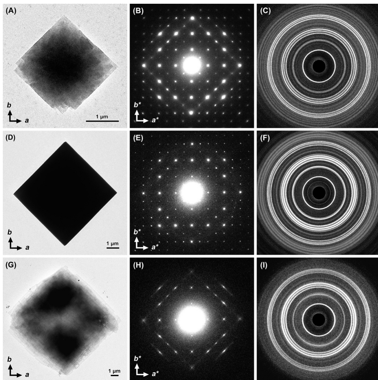
Figure 1. TEM images (A,D,G), base-plane ED patterns (B,E,H) and XRD diagrams (C,F,I) of V-amylose crystals corresponding to the V8 II allomorph: (A–C) V NAP1 (DP130, mixing at 75 °C, no incubation time); (D–F) V SAL (DP60, incubation at 40 °C); (G–I) V QN (DP2500, incubation at 40 °C, 30 vol% DMSO). The ED patterns were recorded at low temperature from frozen-solvated crystals. For clarity, the XRD patterns are those recorded with the laboratory set-up. The composite patterns collected at ESRF are shown in Supporting Information Figure S5 .
