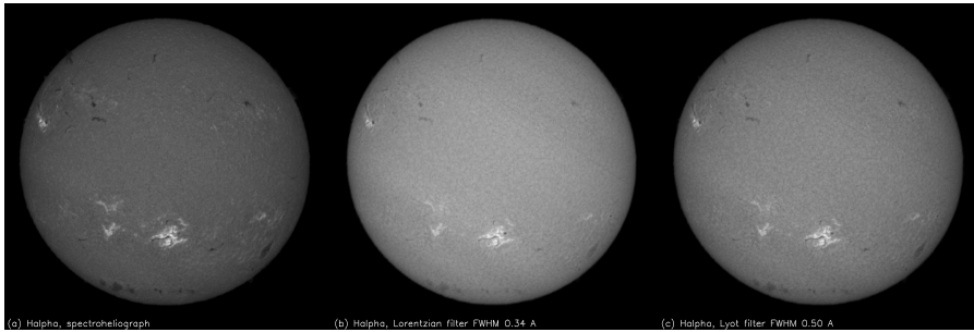
Fig. 12 Simulation of H \alpha images obtained after filtering the (x, y, \lambda) spectroheliograph data-cube. (a) Spectroheliogram at line centre, 28 October 2021. (b) Same image, through a 0.34 Å Lorentzian transmission (such as MTSP filter 2). (c) Same image, with a 0.50 Å five stage Lyot filter, for comparison.
