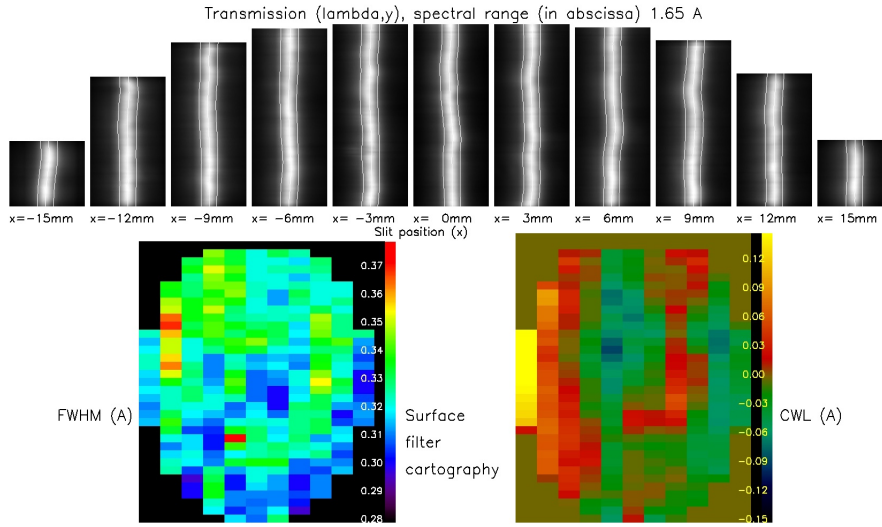
Fig. 10 Calibration of H \alpha filter 2. Top: the H \alpha line through the filter for 11 x-positions of the spectrograph slit (in mm). The white lines delineate the CWL and FWHM (y-direction). Bottom: the filter cartography. The local FWHM (Å) is displayed at left. At right, the CWL (Å) fluctuations are small, so that the integrated bandpass for pupil plane application (0.34 Å) remains narrow.
