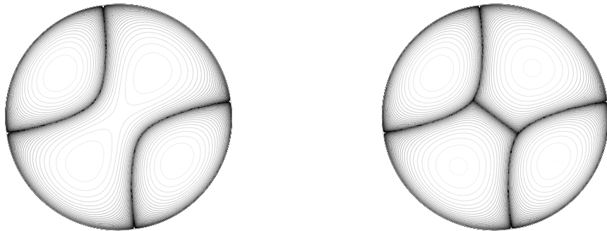
FIGURE 2. Optimal partition and eigenfunctions for (1.6).
