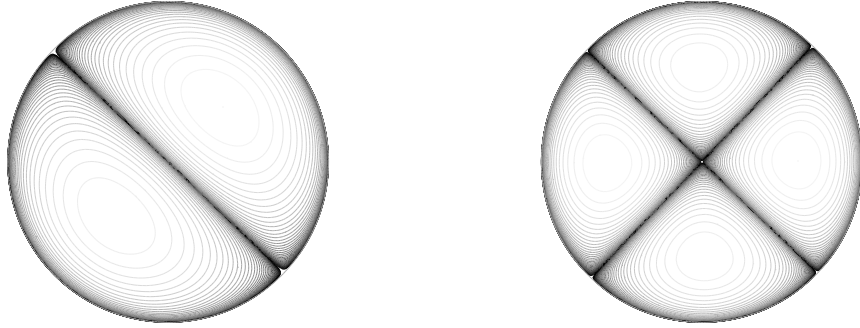
FIGURE 1. Optimal partition and eigenfunctions for (1.5).
