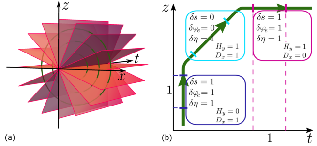
FIG. 1. (a) A t -invariant (electrostatic) case: an Oy charged line with the Ot world line. Green circles: ESs and pink surfaces: ZEFSs. (b) A non- t -invariant case: ES (green line) with purely an electric-field part ( z direction, dark-blue frame), plane-wave part (null-like direction, light-blue frame), and purely magnetic field ( t direction, purple frame). The ES topology is absolute, the interval values \delta s , the flux values \delta \varphi_e , and the characteristic parameter values \delta \eta are all absolute, independent of the reference frame. In contrast, H_y and D_x depend on the axis choice (t, z) with Eqs. (3) and (6). When ES is null-like, only the parameter \eta has a nonzero value, able to describe the electromagnetic field in this region.
