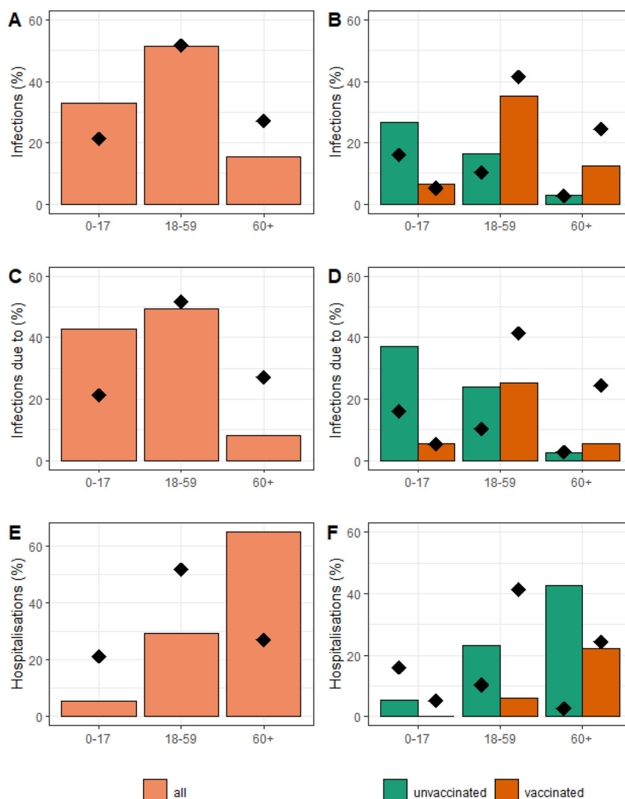
Fig. 1 Contribution of groups defined by their age and vaccination status to infections, disease spread and hospital burden, in our baseline scenario with R_0=5 and a vaccine coverage of 70–80–90% among 12–17 years old, 18–59 years old, and over 60 years old. Age distribution of new infections (A) in the entire population and (B) among vaccinated and unvaccinated individuals. Proportion of infections (C) attributable to different age groups and (D) attributable to different age groups among vaccinated and unvaccinated individuals. Age distribution of hospitalizations (E) in the entire population and (F) among vaccinated and unvaccinated individuals. In all panels, the diamonds indicate the age distribution of the different groups in the population
