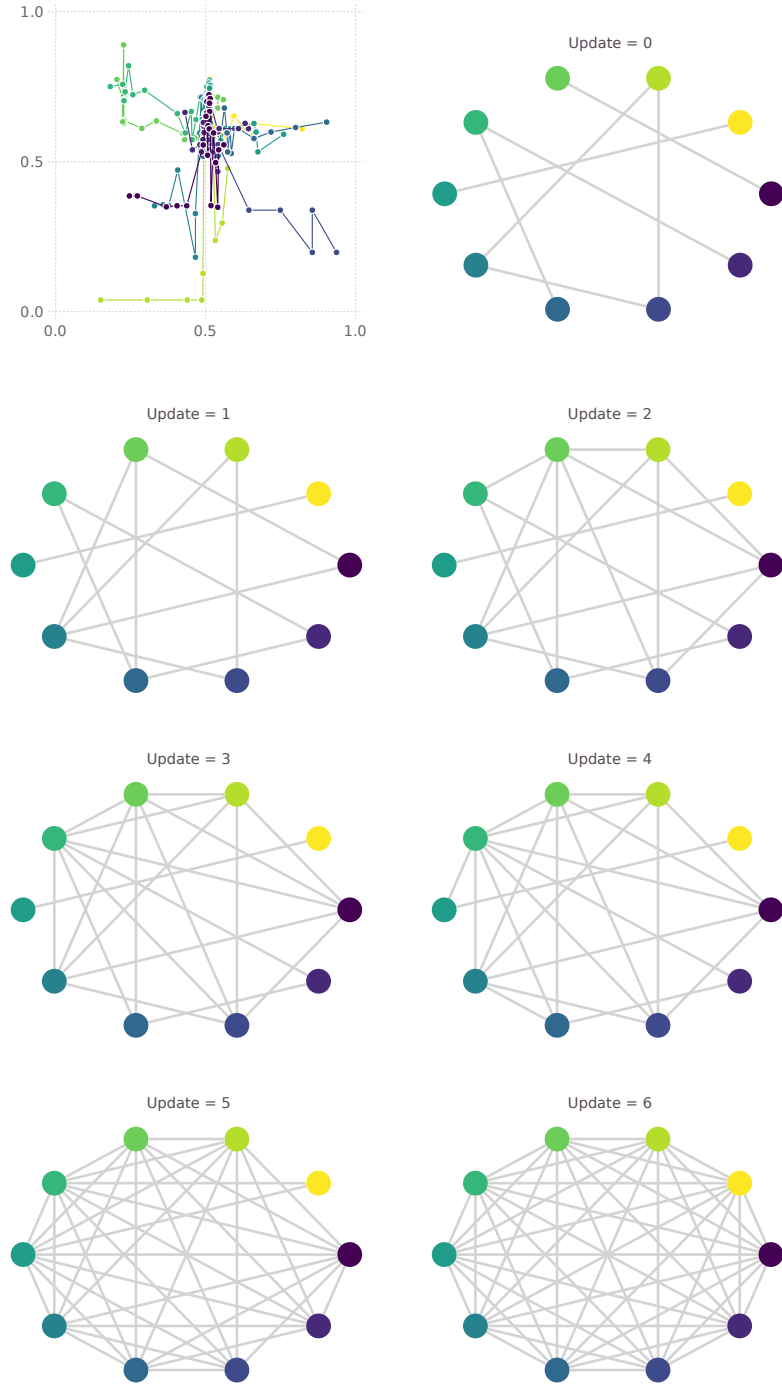
Figure 5: Top left panel showing 20 updates of a community of 10 social Carnapian agents trying to estimate \tau = \langle 0.6, 0.75 \rangle using (BCC) and the proportional choice rule. The other panels show the networks formed by the BCI relations at the first six time steps.
