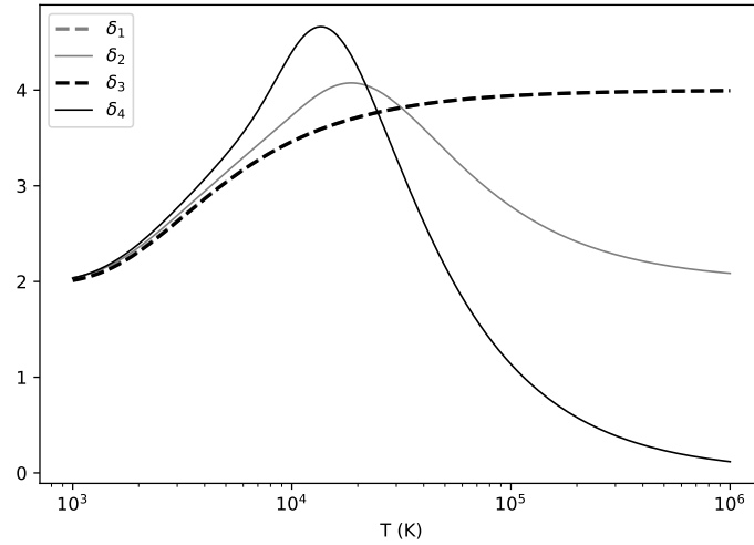
Fig. 2 Number of internal degrees of freedom in the various models at high temperatures.
