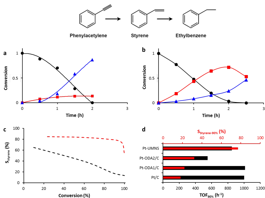
Figure 5. Results of PhA hydrogenation on Pt catalysts. (a) conversion obtained on Pt/C catalyst. (b) conversion obtained on Pt UMNS catalyst (black circles PhA, red squares ST, and blue triangles EB). (c) styrene selectivity evolution with conversion for the Pt/C (black trace) and Pt UMNS catalysts (red trace) and (d) performances of the investigated catalysts at 90% conversion.
