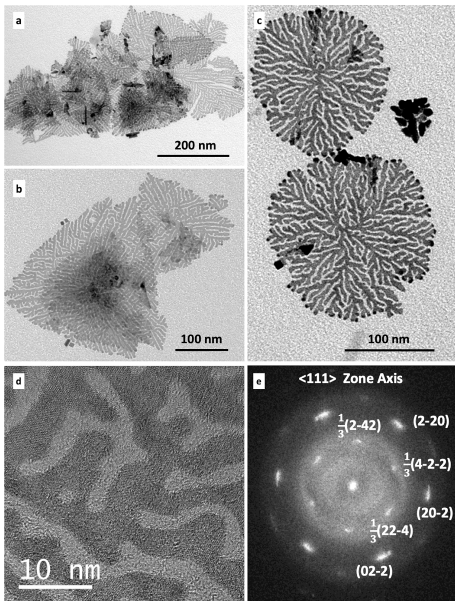
Figure 3. Dendritic Pt UMNS produced after 4 days reaction. (a) Lower magnification image: the UMNS overlap, and folded UMNS appear as higher contrast areas. (b) image of triangularly shaped overlapping nanosheets. (c) round contour Pt UMNS. (d) HRTEM of a UMNS. (e) the corresponding FFT indicating the spots due to the {220} reflections and the spots of the \frac{1}{3} {422} forbidden reflexions.
