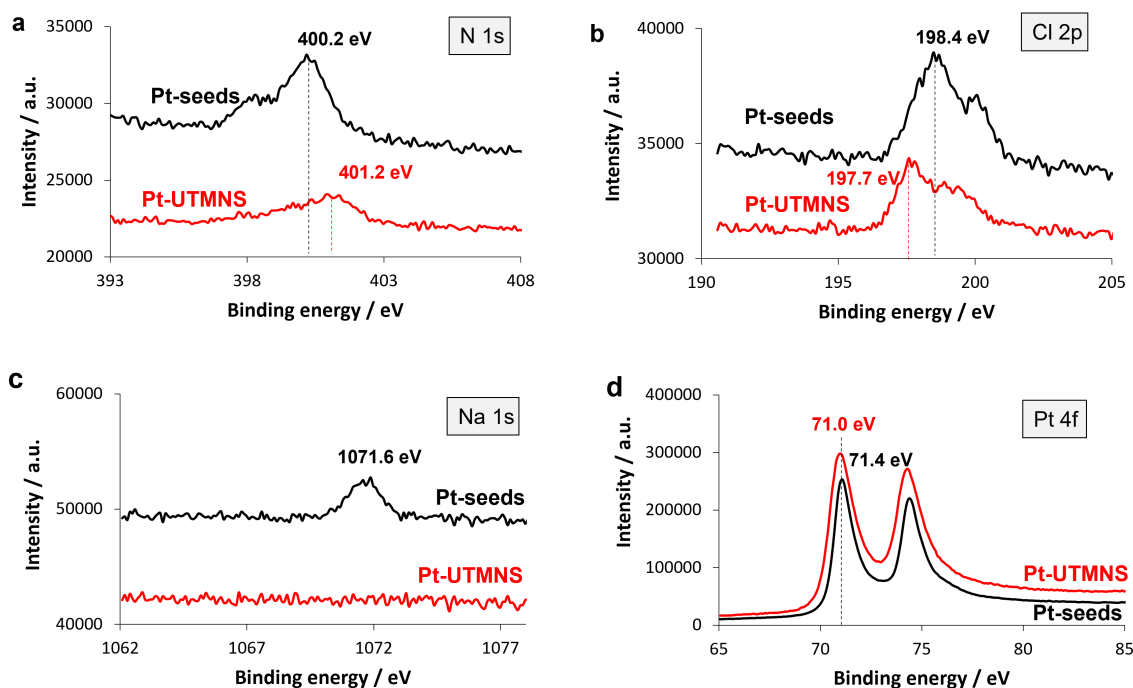
Figure 4. XPS spectra of Pt UMNS and Pt seeds. (a) XPS spectra in the N 1s region. (b) XPS spectra in the Cl 2p region. (c) XPS spectra in the Na 1s region and (d) XPS spectra in the Pt 4f region.
