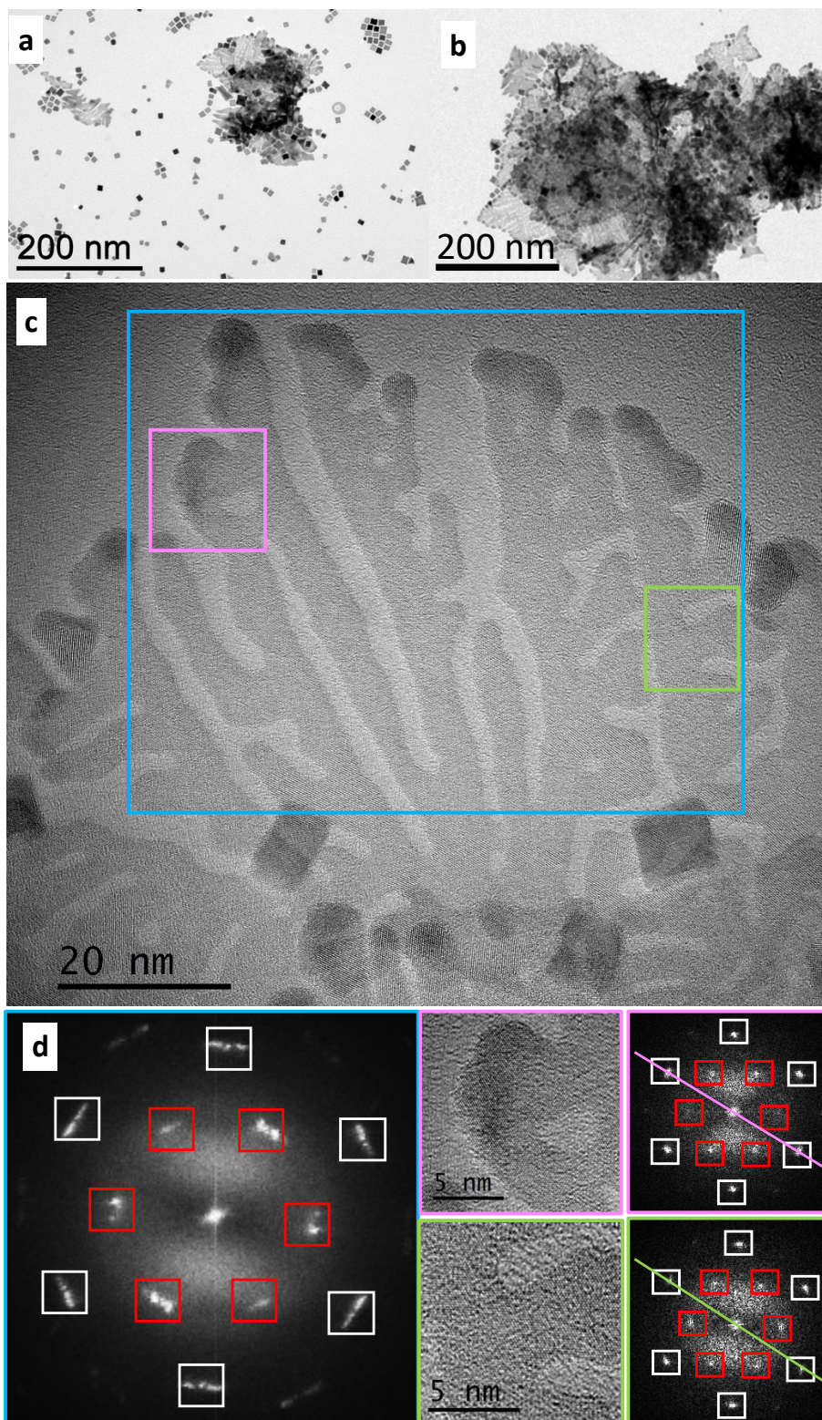
Figure 1. Nanostructures obtained by reduction by \text{H}_2 (3 bar) of \text{Pt}(\text{acac})_2 in the presence of ODA at 20 °C. (a) 4 days reaction. (b) 7 days reaction. (c) HRTEM image of a Pt UMNS obtained after 7 days reaction and (d) FFT of the areas made
