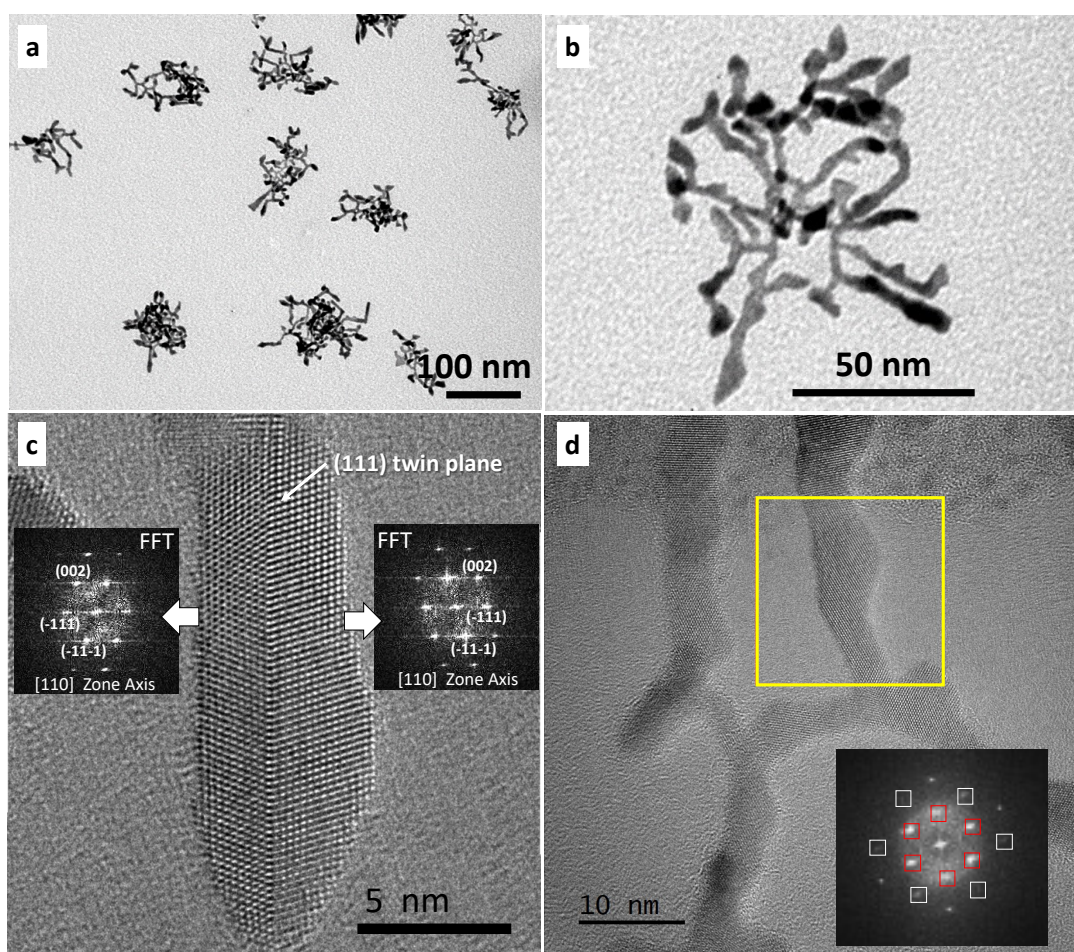
Figure 2. Electron microscopy of multipods resulting after 24 h reduction by \text{H}_2 (3 bar) of \text{PtCl}_2 at 20^\circ\text{C} , in the presence of ODA and \text{Na}(\text{acac}) . (a) general view. (b) an isolated nano-object at higher magnification. (c) HRTEM micrograph of a branch
