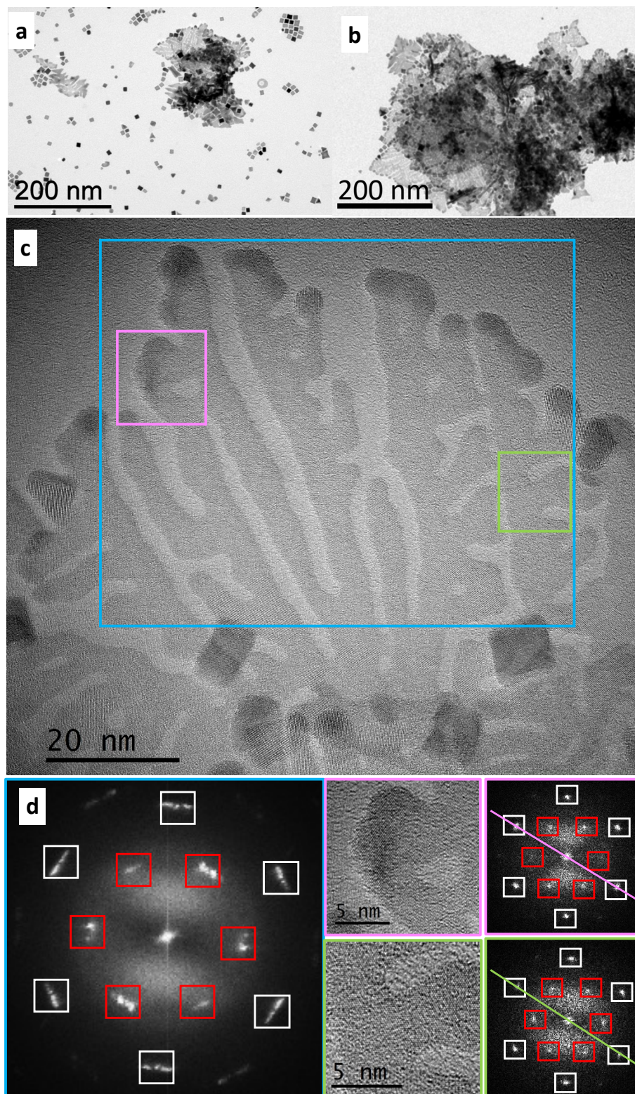
Figure 1. Nanostructures obtained by reduction by \text{H}_2 (3 bar) of \text{Pt}(\text{acac})_2 in the presence of ODA at 20^\circ\text{C} . (a) 4 days reaction. (b) 7 days reaction. (c) HRTEM image of a Pt UMNS obtained after 7 days reaction and (d) FFT of the areas made
