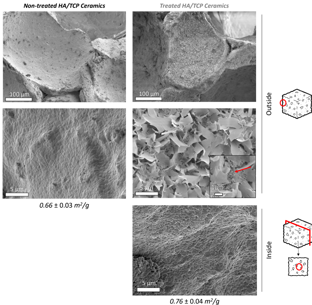
Figure 3. SEM pictures of non-treated and treated (4 h, 37 ^{\circ}\text{C} , 80 bar pressure, L/S = 2) HA/ \beta -TCP ceramic scaffolds and corresponding specific surface area (Krypton BET). Smaller particle sizes around 0.5 \mu\text{m} may be seen on the outer part, with deeper porosity (red arrow).
